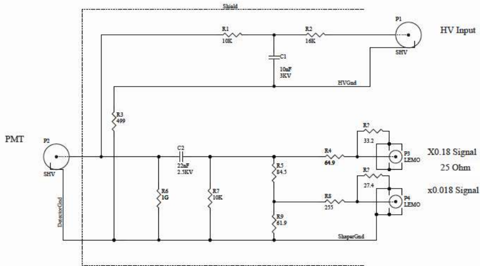
Figure 37. The “splitter” circuit. The circuit connects the HV source to the PMT. It also provides a pathway for signal pulses from the PMT to reach the readout electronics via an AC-coupling capacitor (C2). The signal is split into two copies, one provided with an attenuation factor of 0.18 and another at 0.018. Both signal sources are recorded by the readout electronics in order to provide two dynamic ranges.
