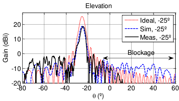
Fig. 9 Measured (Meas) and simulated (Sim) elevation radiation patterns at 100 GHz for the beam scanned to -25^\circ in elevation. The ideal radiation pattern is also plotted. Simulation considers the actual reflection coefficient of the cells.
