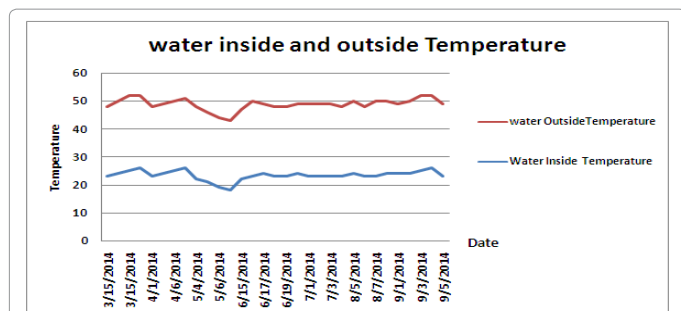
Figure 13: Water outside and inside temperature variation from for a period of six months.
