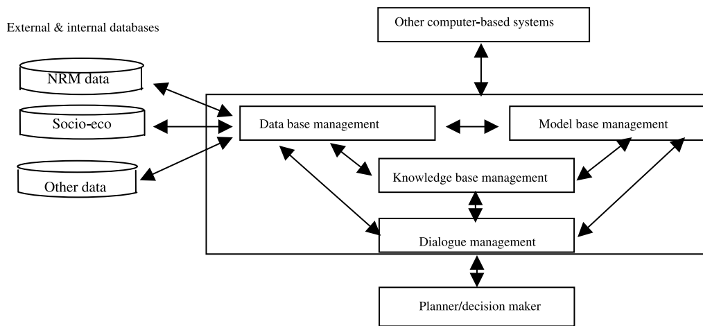
Figure 2 | Overall architect of a planning support system (adapted from Turban 1995).
