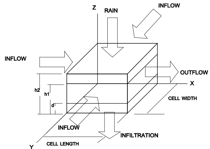
Figure 4 | Element in hydrological modelling at grid scale.
