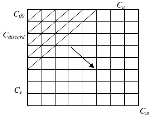
Figure 4: Manner of discarding DCT coefficients (only the first 8x8 coefficients are shown)
