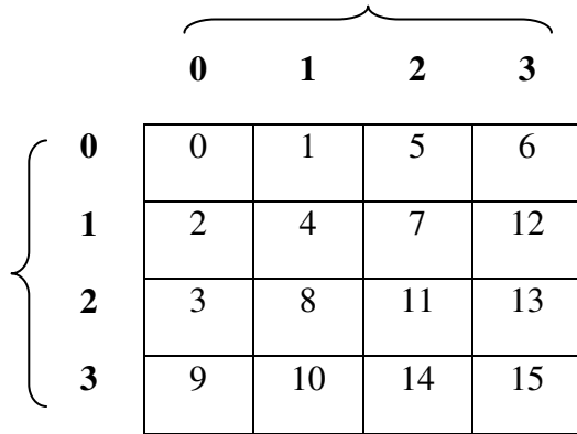
Figure 15: Ordering of 2D DCT coefficients C(v,u) for N_p = 4
