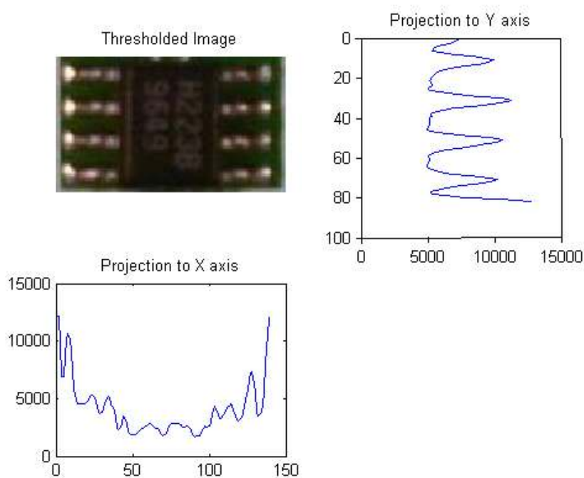
Figure 10: Image processing of solder joint
