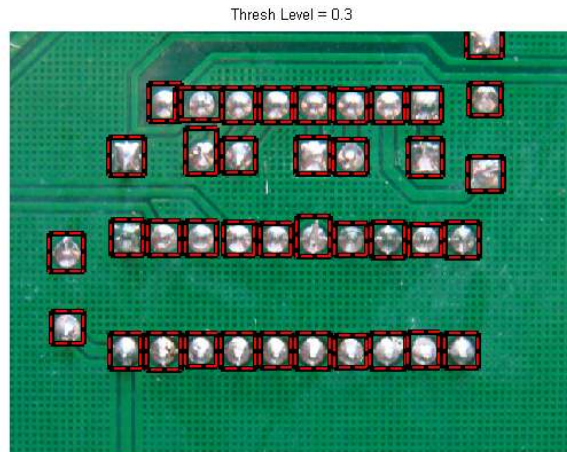
Figure 12: An example of detected solder joints form database 2
