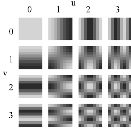
Figure 14: Graphical interpretation of the first few 2D DCT basic function for N=8 ; (lighter colours represent larger value)
