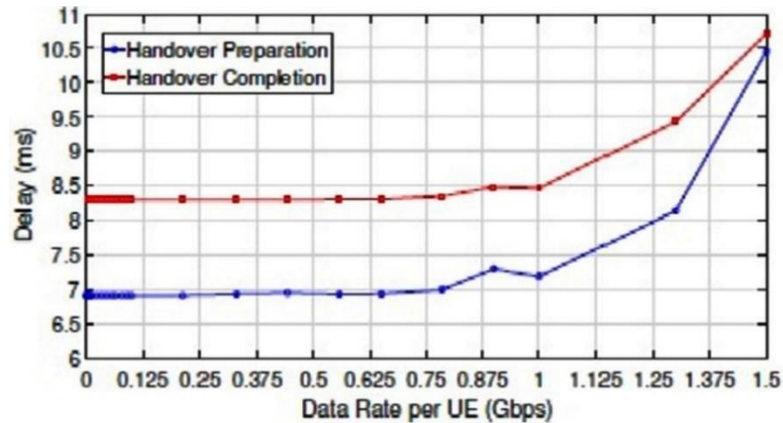
Figure 11. Performance of the handover simulation model on the basis of execution time
