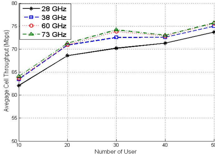
Figure 9. Average rate vs number of user
