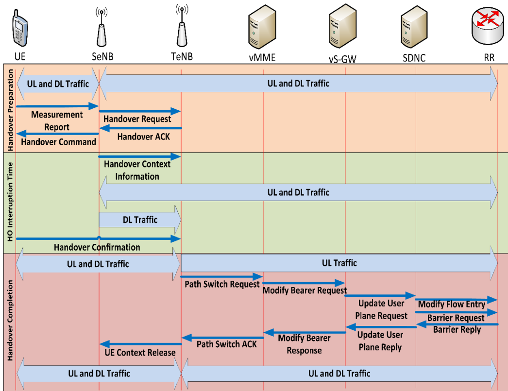
Figure 6. Implemented handover for the 5G simulated network
