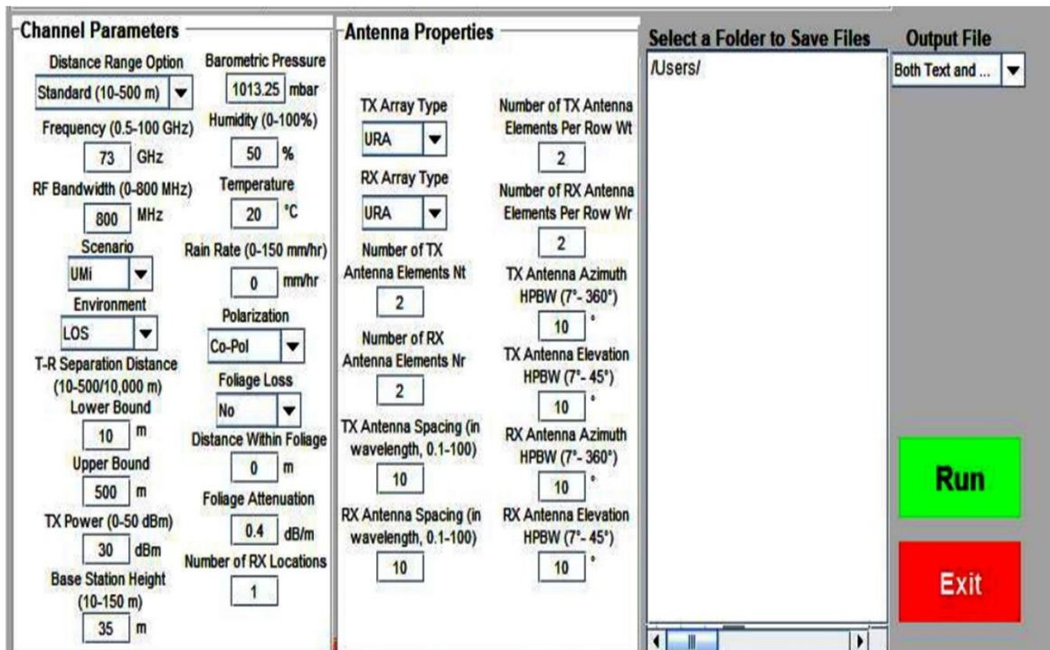
Figure 4. Graphical representation of 5G simulator model
