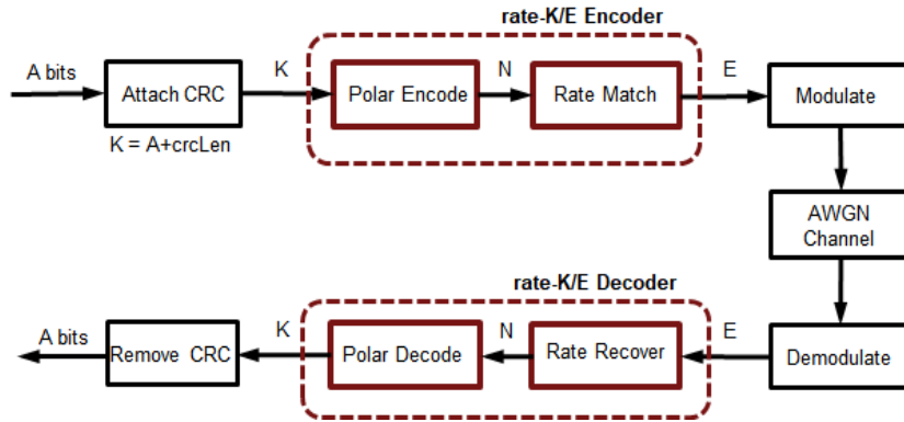
Figure 5. The architecture of channel parameter towards simulation model
