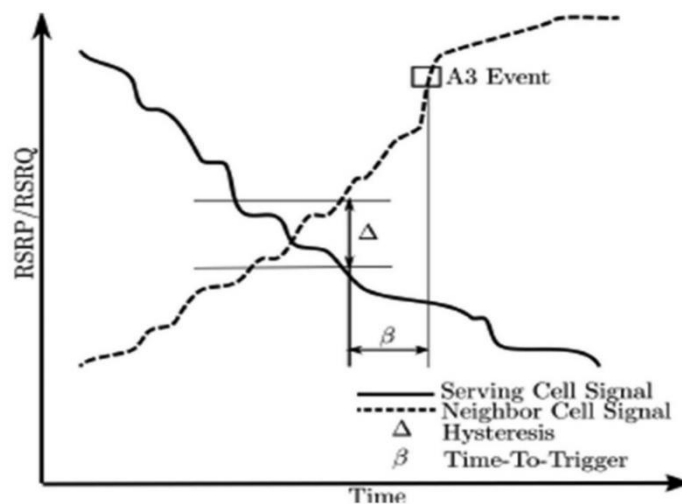
Figure 1. Description of handover mechanism among the cellular network
