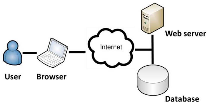
Fig. 7. System development
