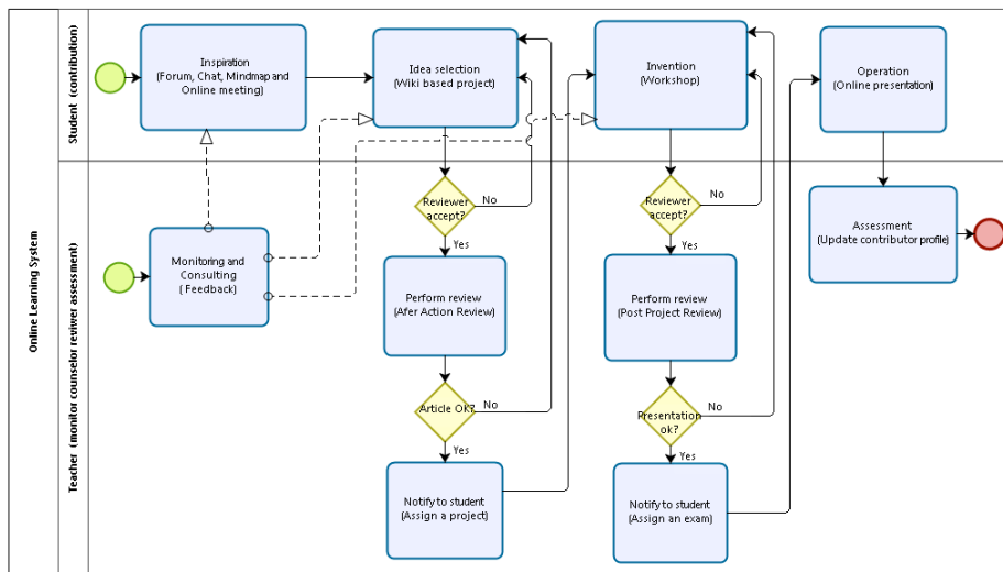
Fig. 5. System diagram
