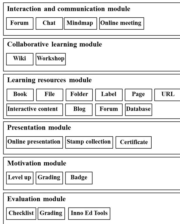
Fig. 6. System architecture
