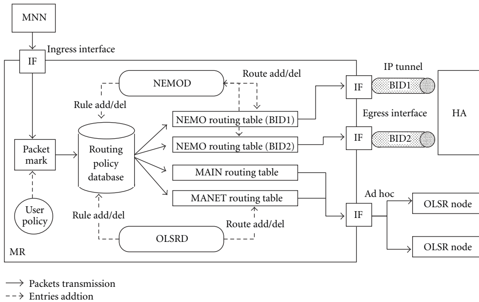
FIGURE 7: Internal route updating and selection mechanisms. NEMO and OLSRD routes are stored in completely independent routing tables.
