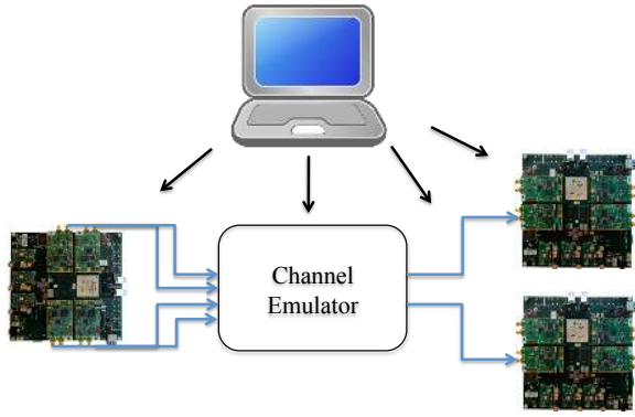
Figure 9: Channel emulator setup.
