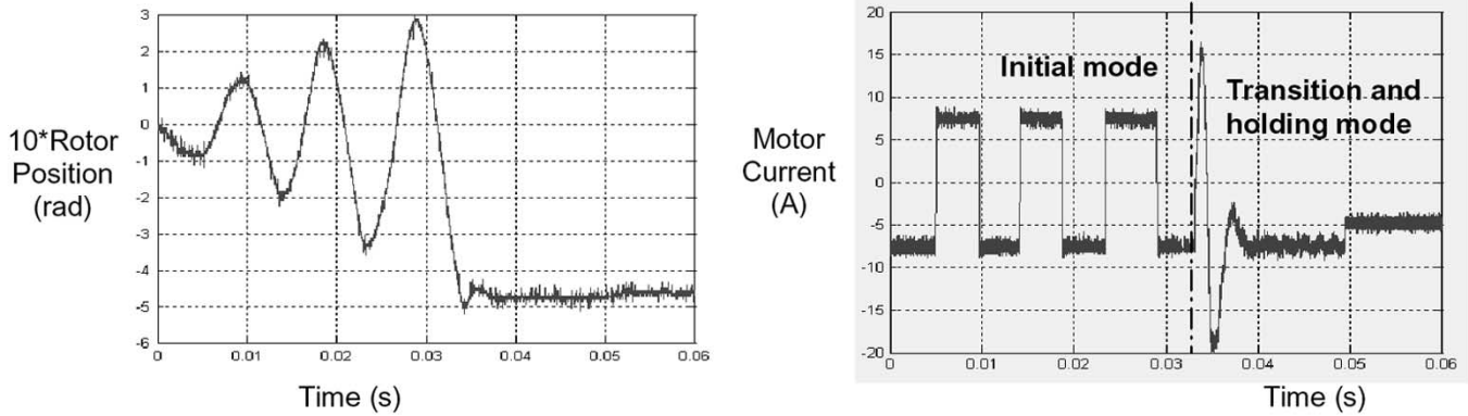
Fig. 11. Experimental waveforms during initial mode control. The initial mode transient was completed in 35 ms with \pm 8 A current pulses, and required an average electrical power of 150 W.
