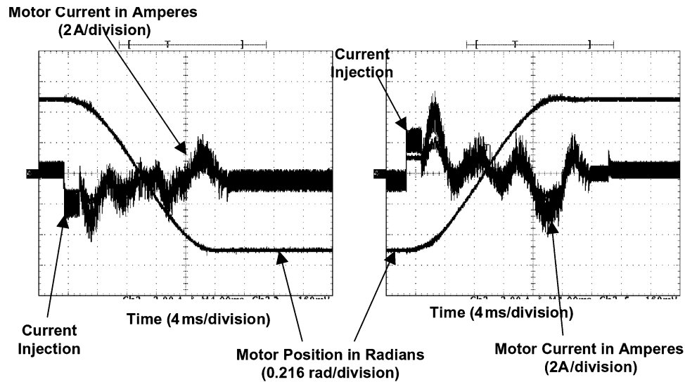
Fig. 12. Experimental results for the transition mode with 12.8 ms transition time.
