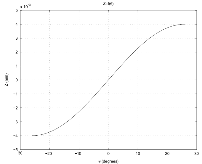
Fig. 3. Desirable transfer characteristic for the nonlinear mechanical transformer. The slope of this profile is the gear ratio of the EMVD when viewed from the \theta domain.
