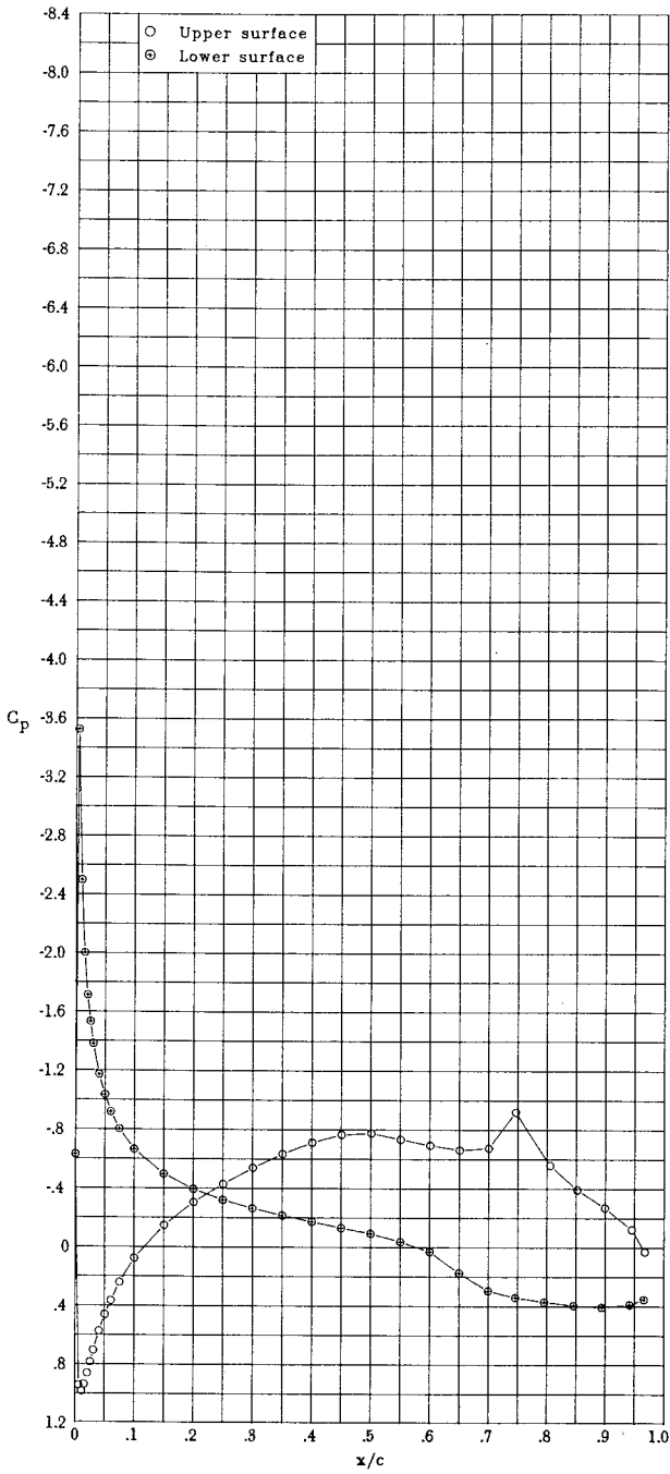
(c) \alpha = -9.11^\circ ; c_l = 0.284 ; c_d = 0.0077 ; c_m = -0.233 .
