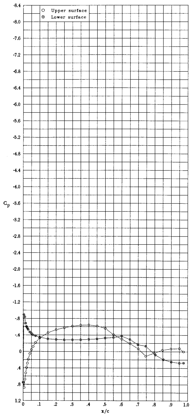
(n) \alpha = 0.48^\circ ; c_l = 0.082 ; c_d = 0.0066 ; c_m = -0.044 .
