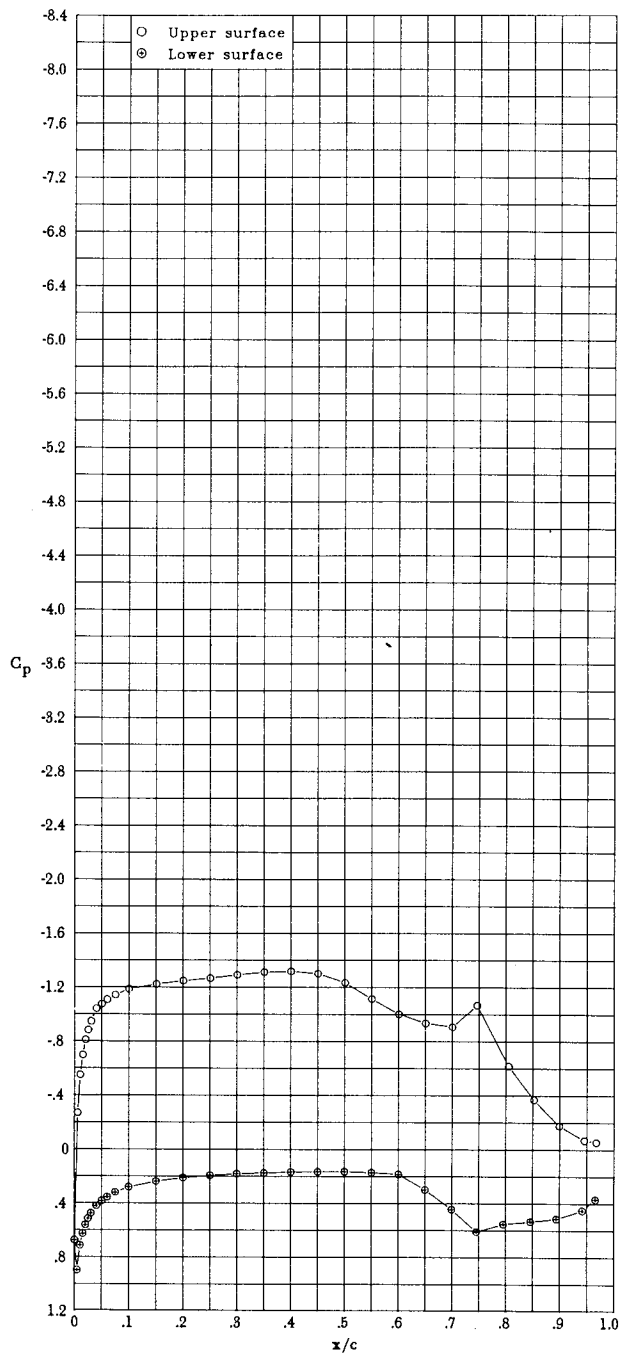
(l) \alpha = 0.05^\circ ; c_l = 1.223 ; c_d = 0.0061 ; c_m = -0.240 .
