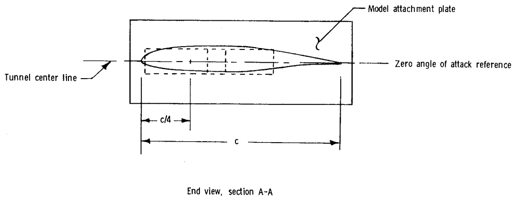
Figure 3.- Typical airfoil model mounted in wind tunnel. All dimensions are in terms of model chord, c = 61.0 \text{ cm} (24.0 \text{ in.}) .
