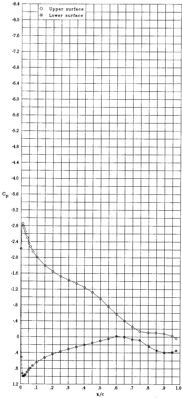
(aa) \alpha = 11.17^\circ ; c_l = 1.229 ; c_d = 0.0106 ; c_m = -0.059 .
