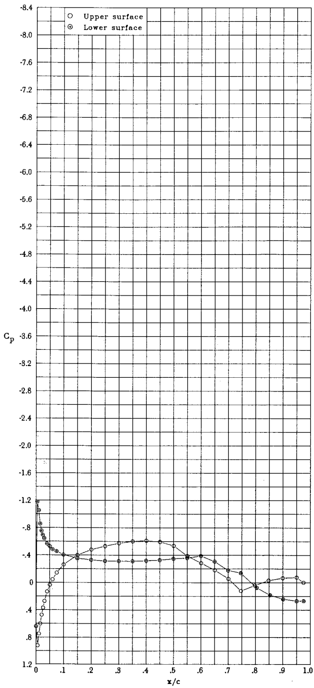
(m) \alpha = -0.02^\circ ; c_l = 0.027 ; c_d = 0.0069 ; c_m = -0.043 .
