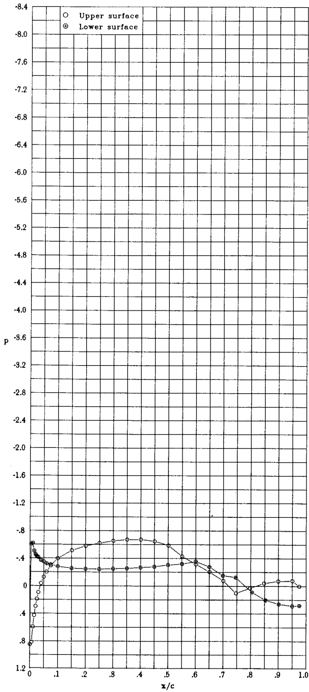
(o) \alpha = 1.00^\circ ; c_l = 0.142 ; c_d = 0.0084 ; c_m = -0.045 .
