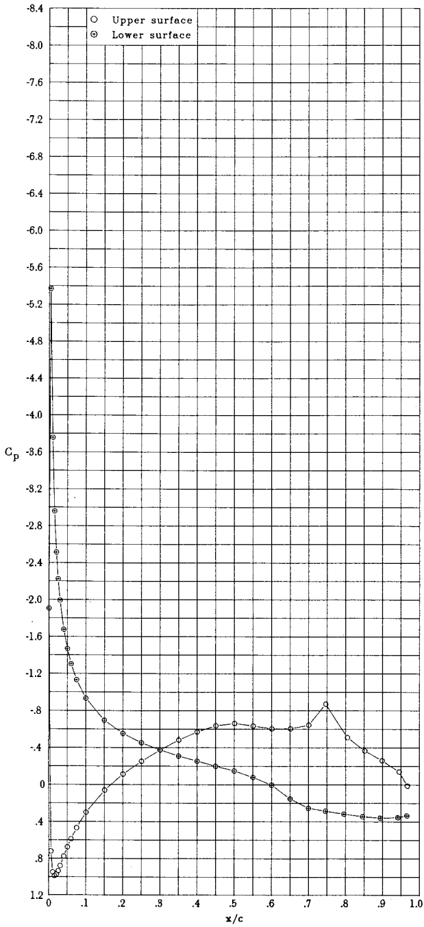
(a) \alpha = -11.18^\circ ; c_l = 0.059 ; c_d = 0.0084 ; c_m = -0.228 .
