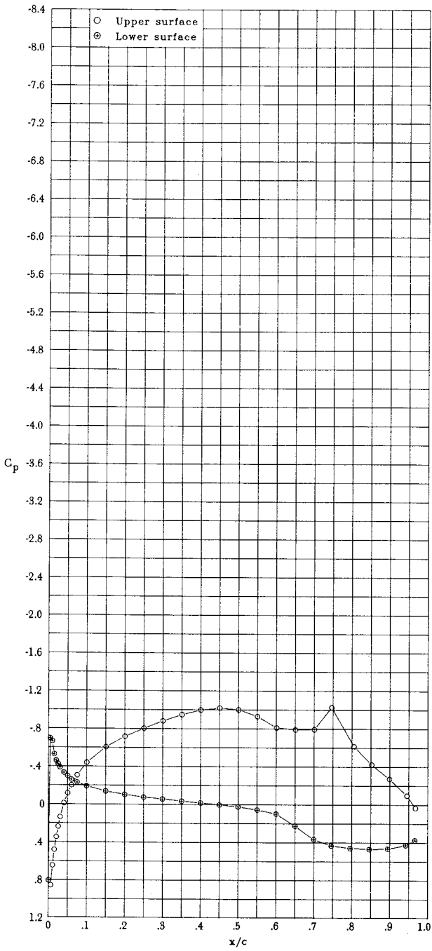
(g) \alpha = -5.04^\circ ; c_l = 0.721 ; c_d = 0.0068 ; c_m = -0.240 .
