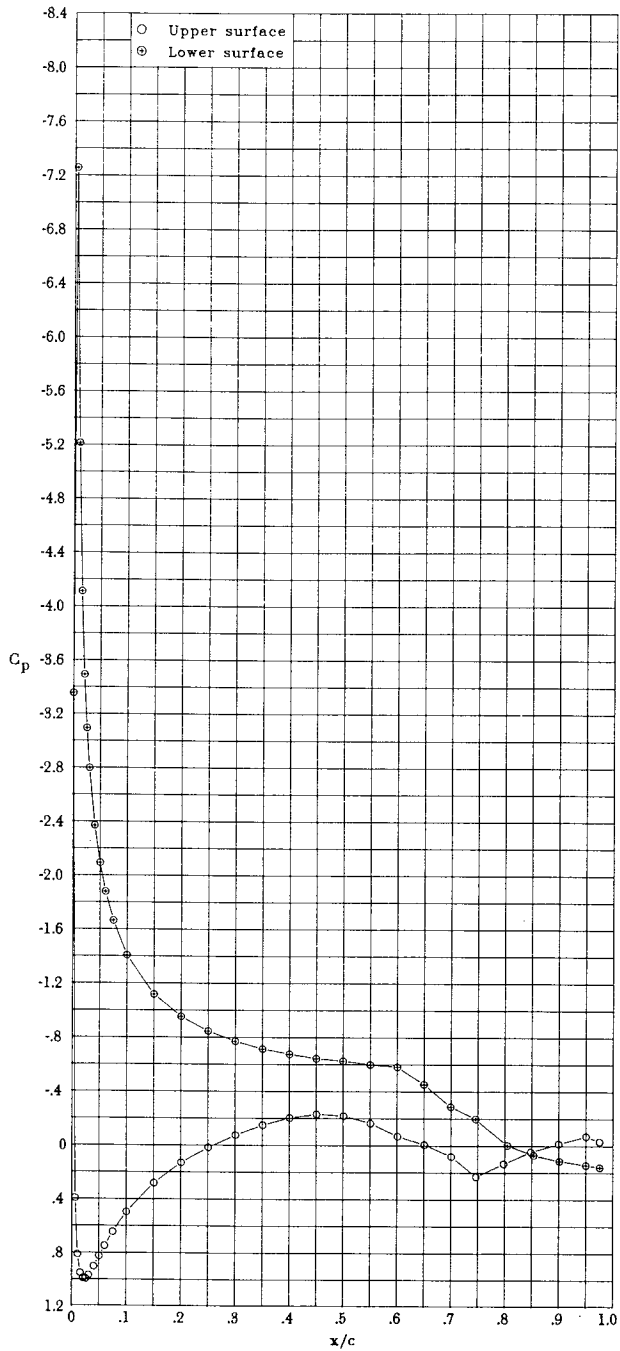
(e) \alpha = -7.13^\circ ; c_l = -0.749 ; c_d = 0.0131 ; c_m = -0.035 .
