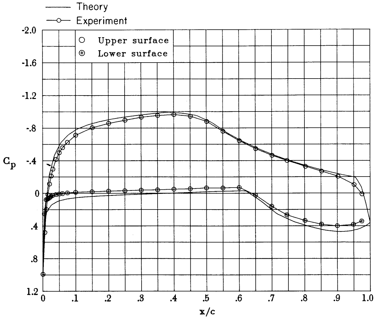
(a) \delta_f = 0^\circ ; \alpha = 0.01^\circ .
