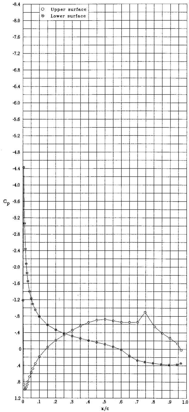
(b) \alpha = -10.12^\circ ; c_l = 0.180 ; c_d = 0.0083 ; c_m = -0.232 .
