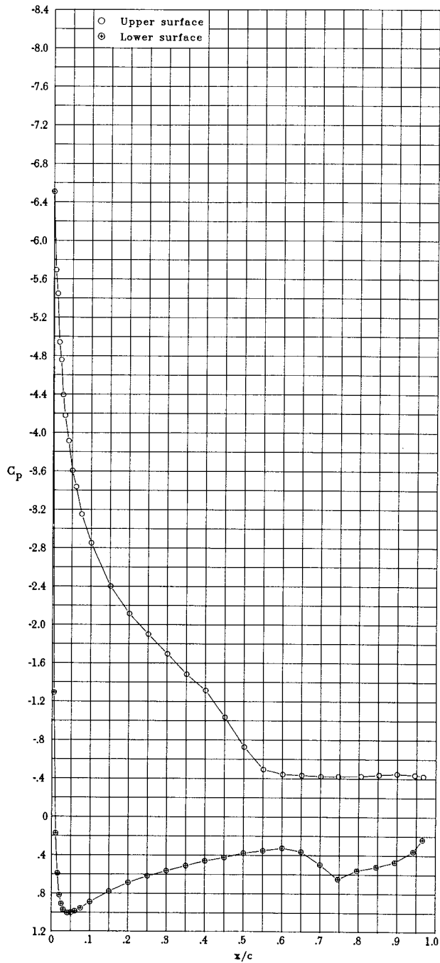
(z) \alpha = 14.21^\circ ; c_l = 1.745 ; c_d = 0.1312 ; c_m = -0.133 .
