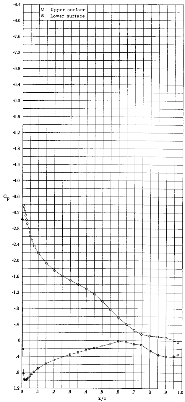
(bb) \alpha = 12.16^\circ ; c_l = 1.325 ; c_d = 0.0122 ; c_m = -0.059 .
