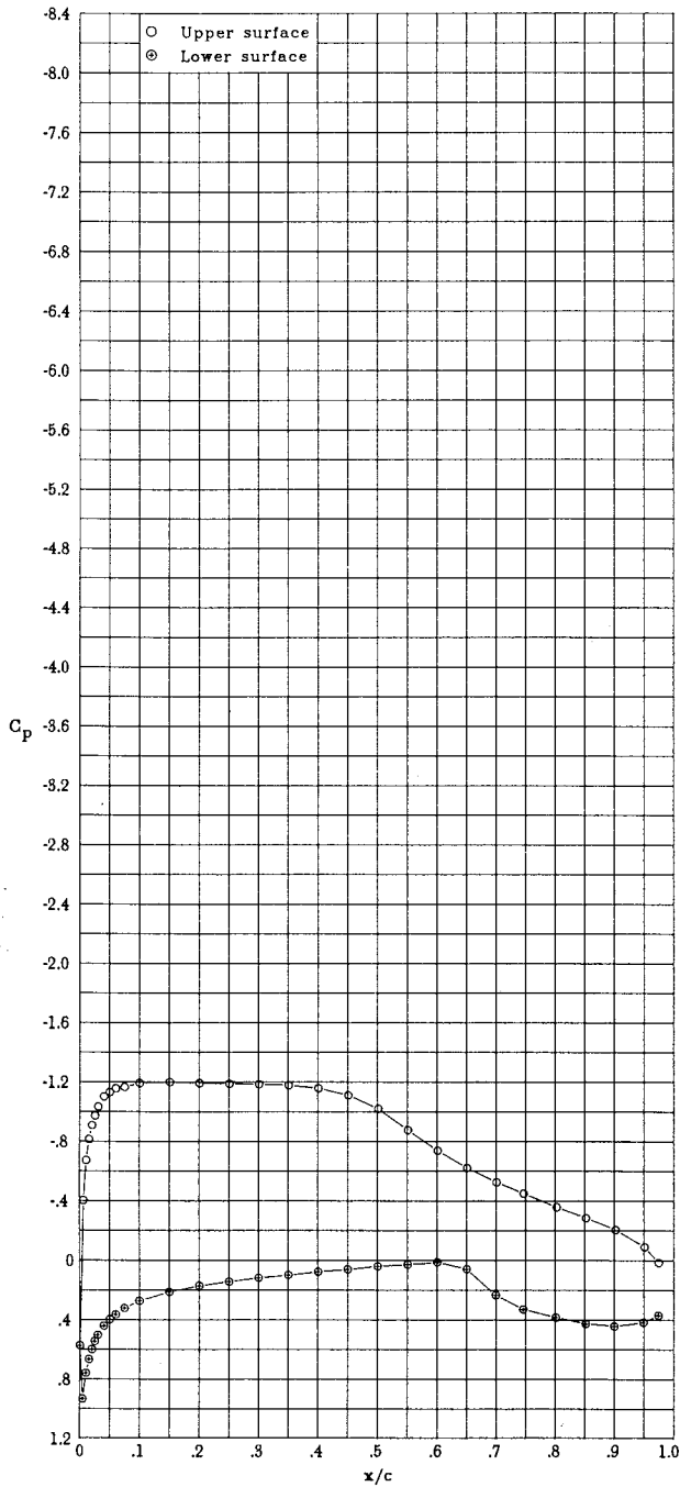
(q) \alpha = 3.06^\circ ; c_l = 0.981 ; c_d = 0.0057 ; c_m = -0.152 .
