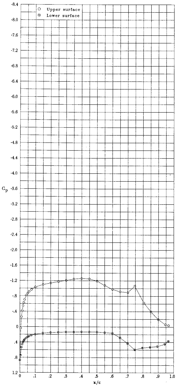
(k) \alpha = -0.98^\circ ; c_l = 1.129 ; c_d = 0.0059 ; c_m = -0.242 .
