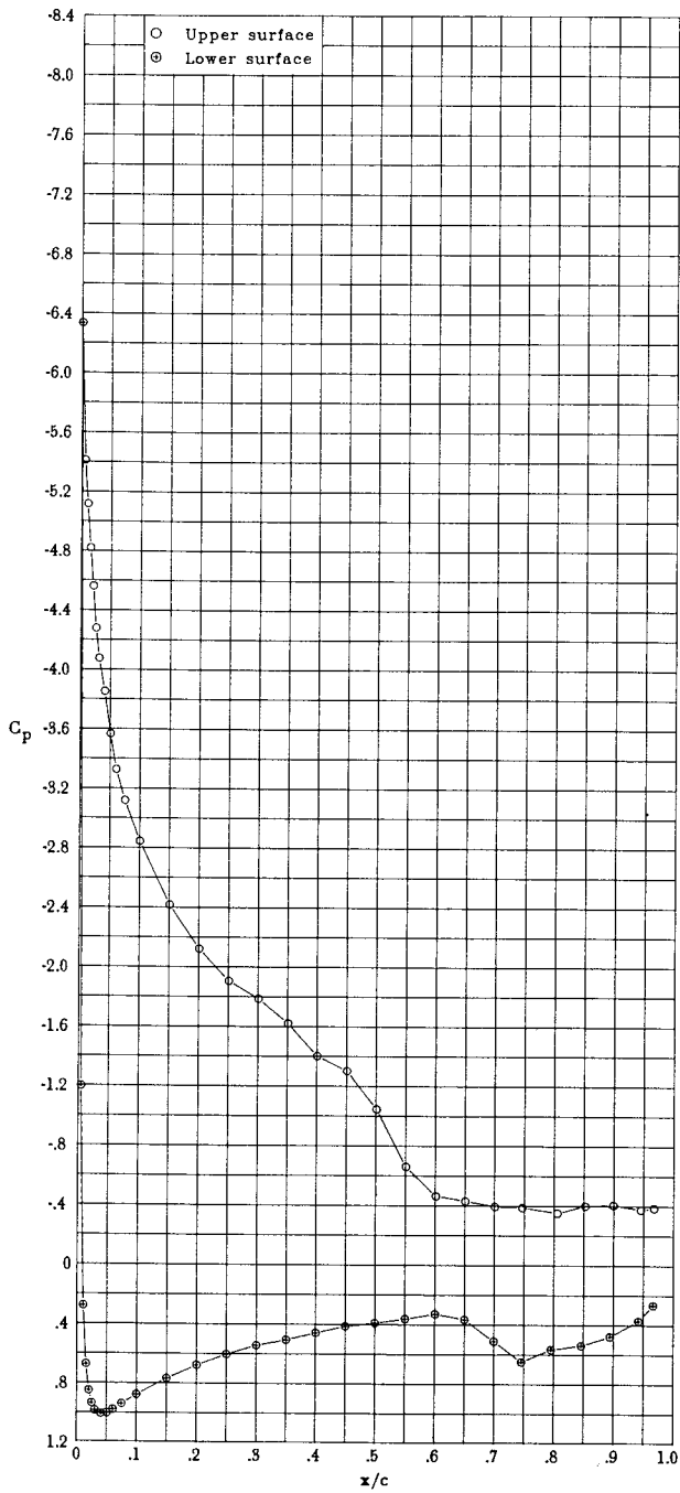
(y) \alpha = 13.20^\circ ; c_l = 1.786 ; c_d = 0.1039 ; c_m = -0.140 .
