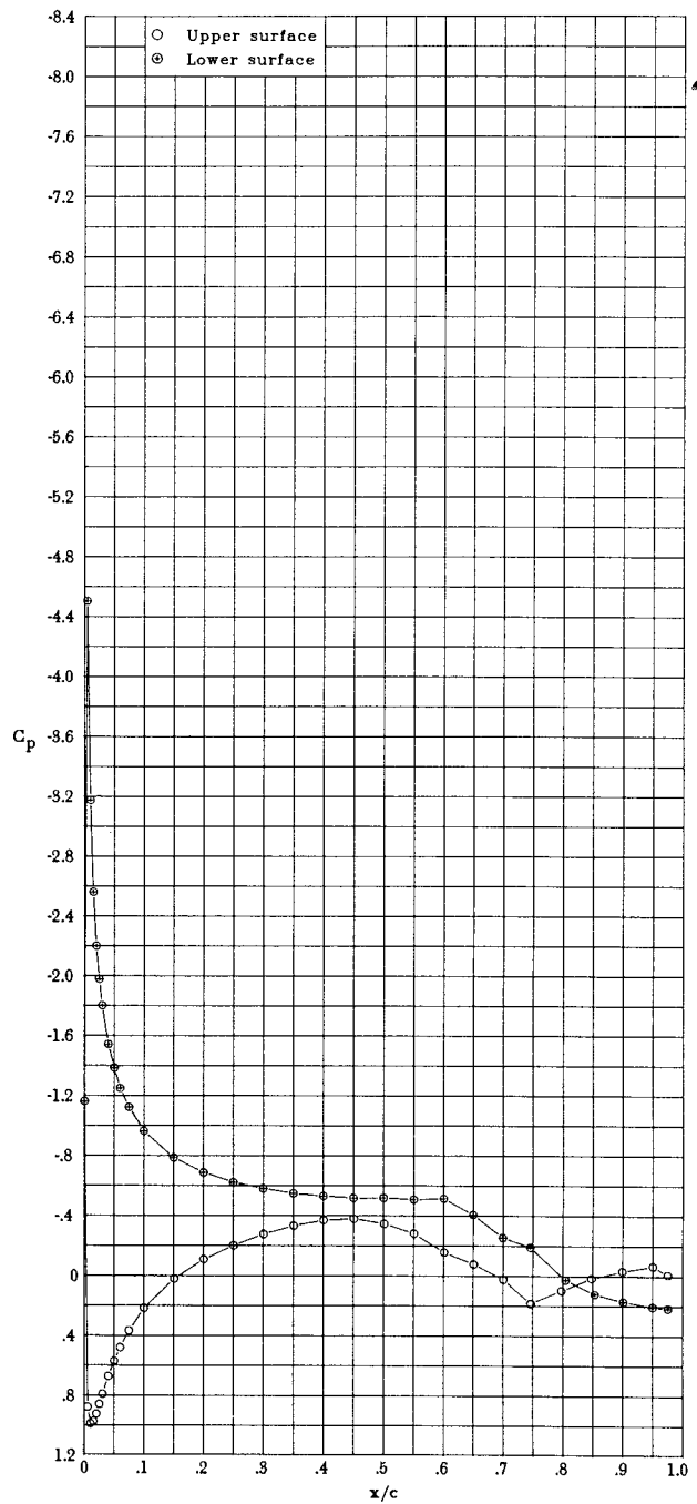
(h) \alpha = -4.10^\circ ; c_l = -0.431 ; c_d = 0.0091 ; c_m = -0.037 .
