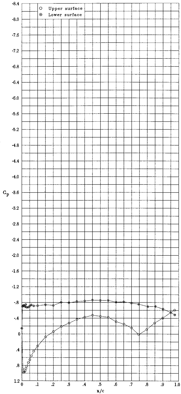
(b) \alpha = -10.10^\circ ; c_l = -0.522 ; c_d = 0.2036 ; c_m = 0.068 .
