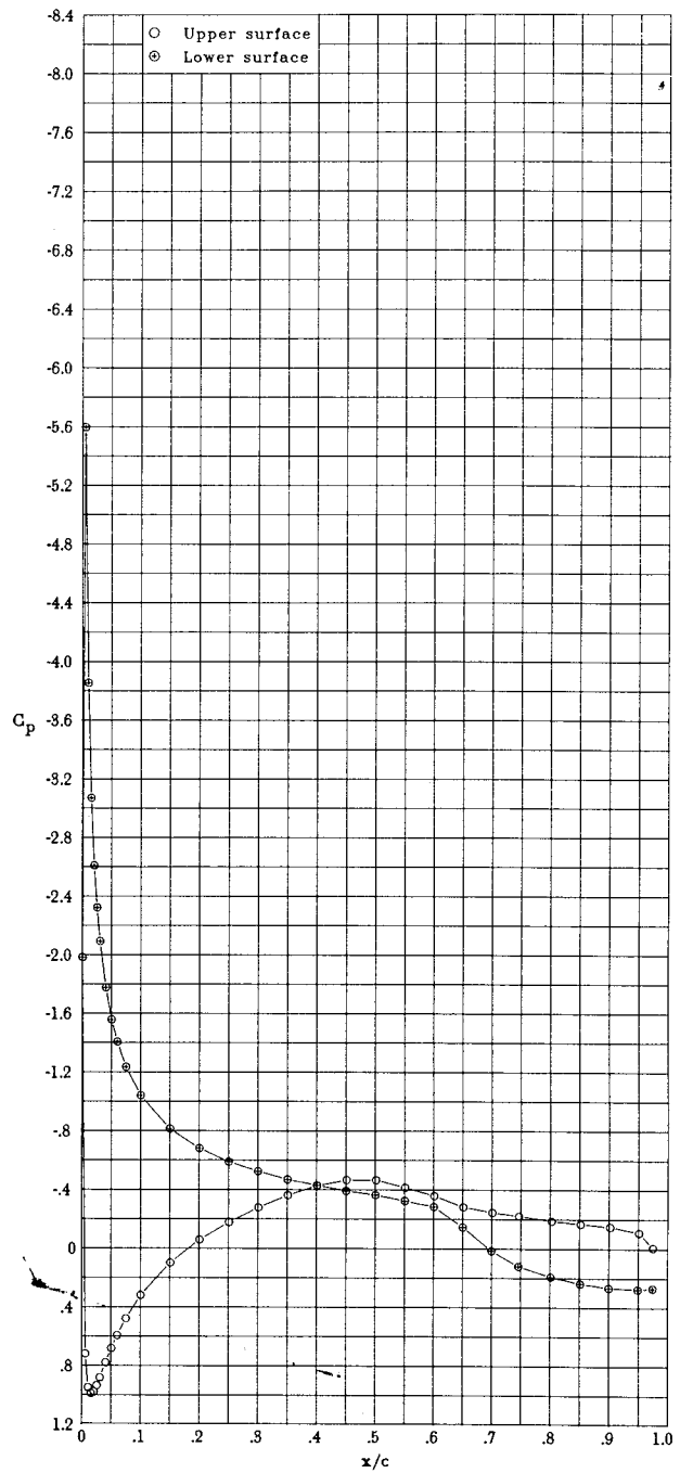
(f) \alpha = -8.15^\circ ; c_l = -0.284 ; c_d = 0.0090 ; c_m = -0.130 .
