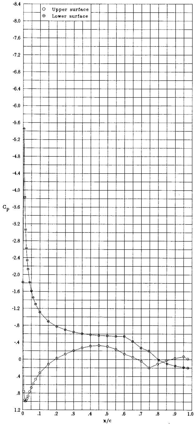
(g) \alpha = -5.11^\circ ; c_l = -0.541 ; c_d = 0.0104 ; c_m = -0.036 .
