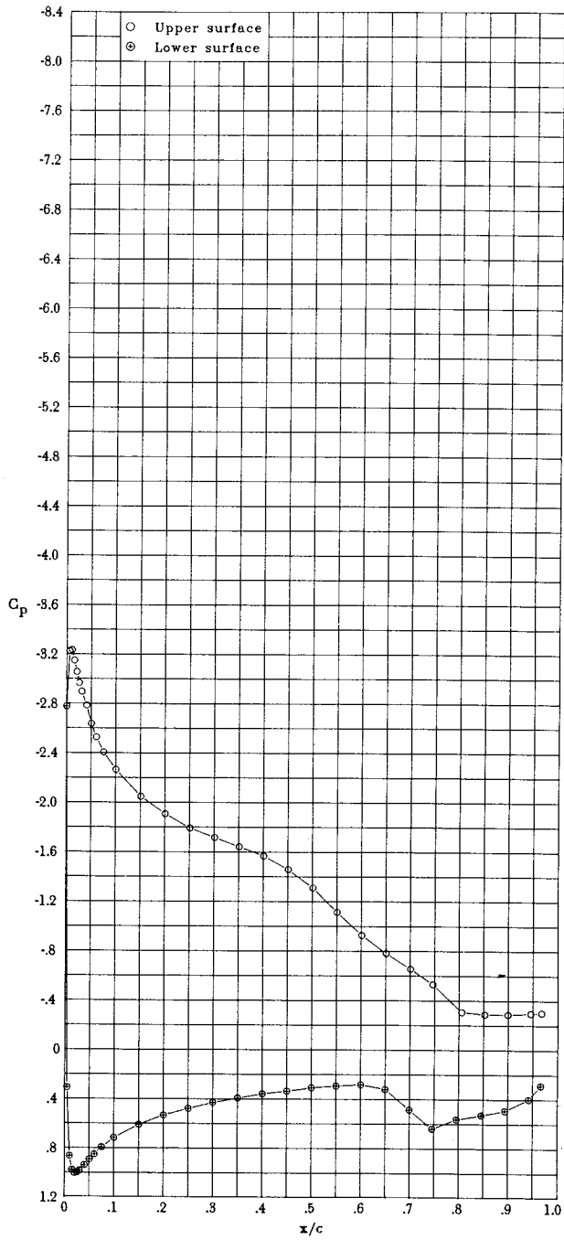
(t) \alpha = 8.14^\circ ; c_l = 1.674 ; c_d = 0.0358 ; c_m = -0.184 .
