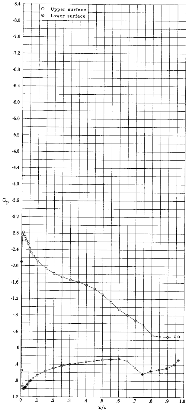
(s) \alpha = 7.13^\circ ; c_l = 1.612 ; c_d = 0.0338 ; c_m = -0.189 .
