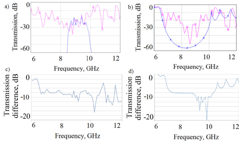
Figure 7. (a) Simulated transmission through the line containing 20 unit cells in the presence of the non-ideal (rf-leaky) sample holder (magenta) and simulation for an ideal (no-leak) sample holder (blue) for a value of \cos \varphi = 0.8 . (b) Same data and color coding as in (a), but with \cos \varphi = 0.2 . (c) Expected response to magnetic field (from \cos \varphi = 0.2 to 0.8 ) for the leaky holder as the difference between in transmission (a) and (b). (d) The same difference as in (c) but with an ideal sample holder.
