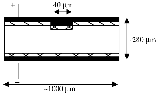
Fig. 2. Cross-section of bulk silicon temperature sensor.
