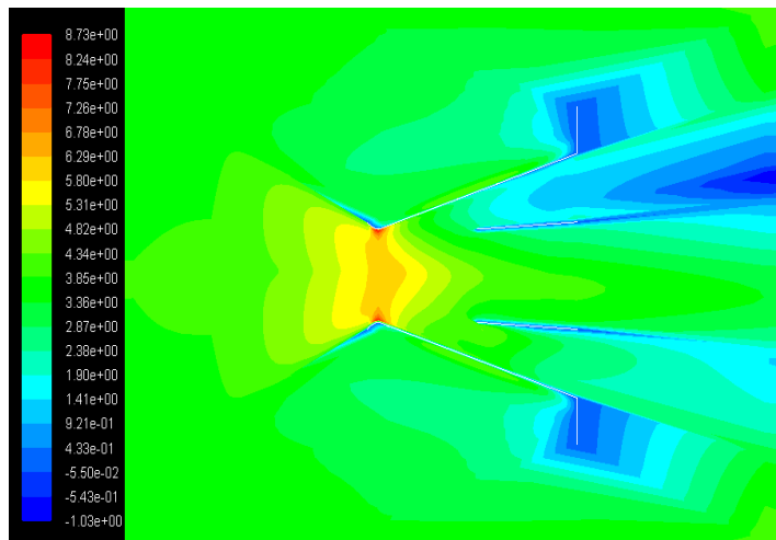
Fig. 14. Re-developed Design (Concept 4) - The Wind Velocity Contour for L_1=0.5 m and \alpha_1=4^\circ .
