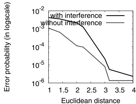
Figure 3: Fast decay in probability of erroneous decoding as the distance between the correct symbol and the erroneously decoded symbol increases. Data based on 10 million known 64-QAM symbols transmitted. In the ambient noise scenario, the overall BER was 3 \times 10^{-4} . In the explicit interference scenario, the overall BER was 6 \times 10^{-3} .
