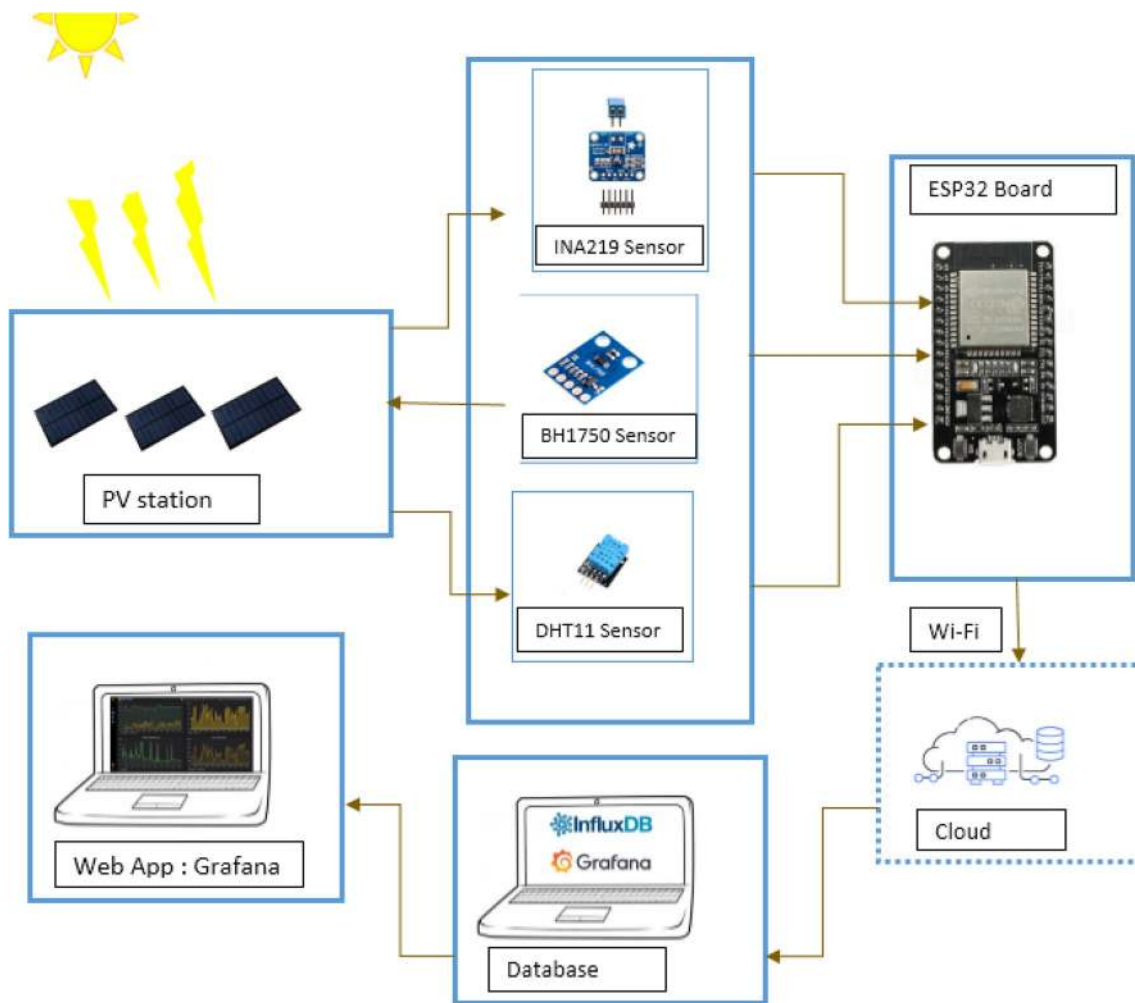
Fig. 1 Block diagram of the overall system
