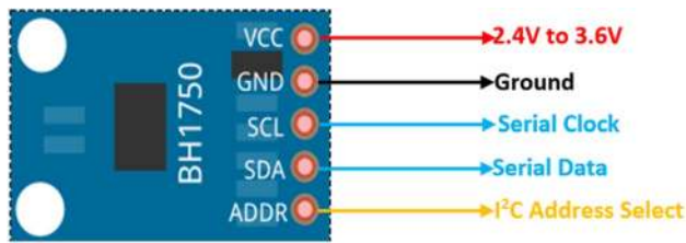
Fig. 5 The Luminosity sensor BH1750
