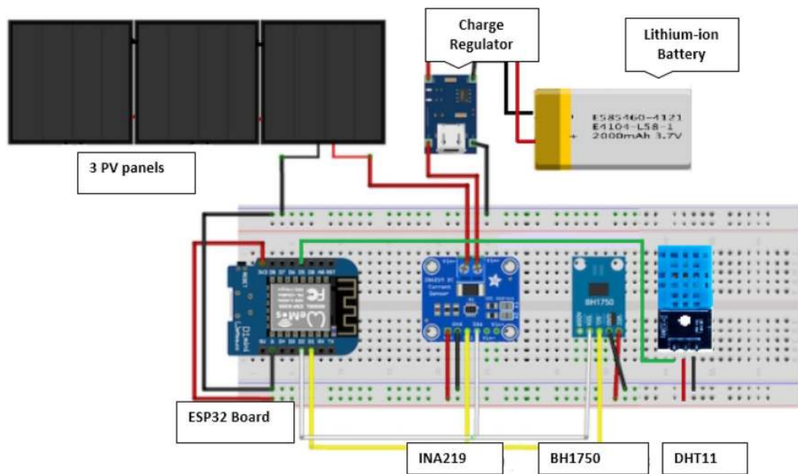
Fig. 2 The experimental setup of the system
