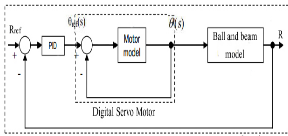
Figure 6. Overall system
