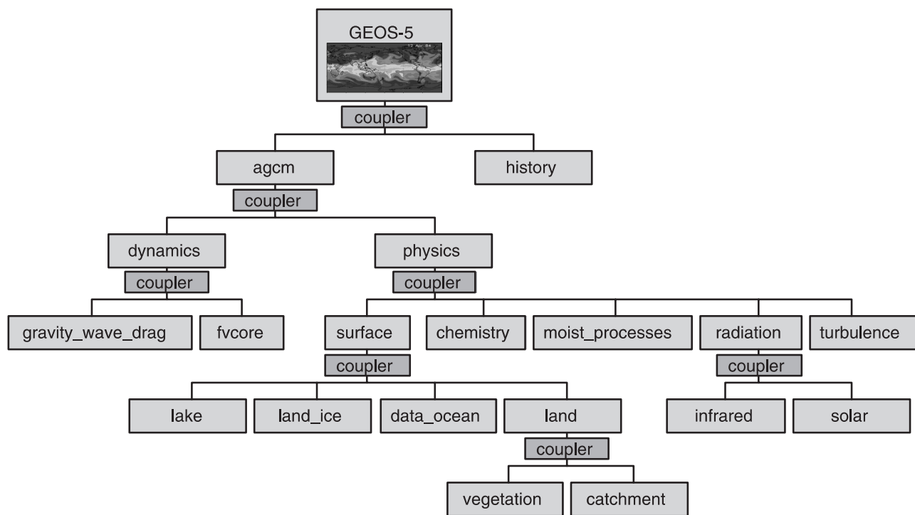
Fig. 2 ESMF-based architecture of the GEOS-5 atmospheric general circulation model. Each box is an ESMF component. Component and coupling interfaces are standardized to facilitate exchanges and extensions. The operations in each component or coupling transformation can be easily customized.
