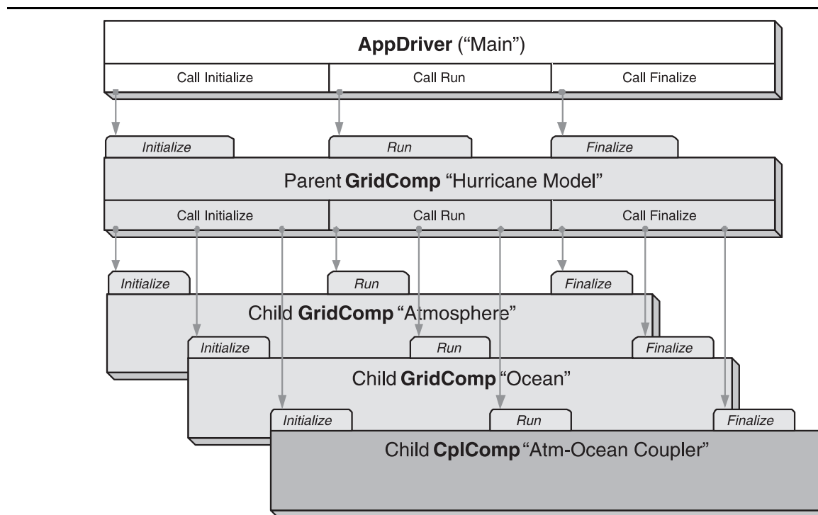
Fig. 1 Application example showing two ESMF gridded components (atmosphere and ocean) and a coupler component. These are the child components of a gridded component that simulates hurricanes. The entire assemblage is called by an application driver.
