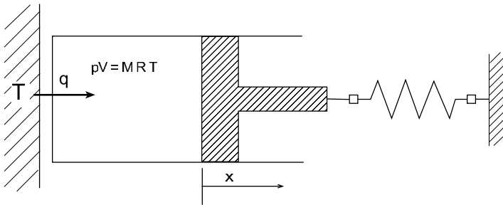
Figure 2.1 Coupling of thermodynamic control volume and piston
