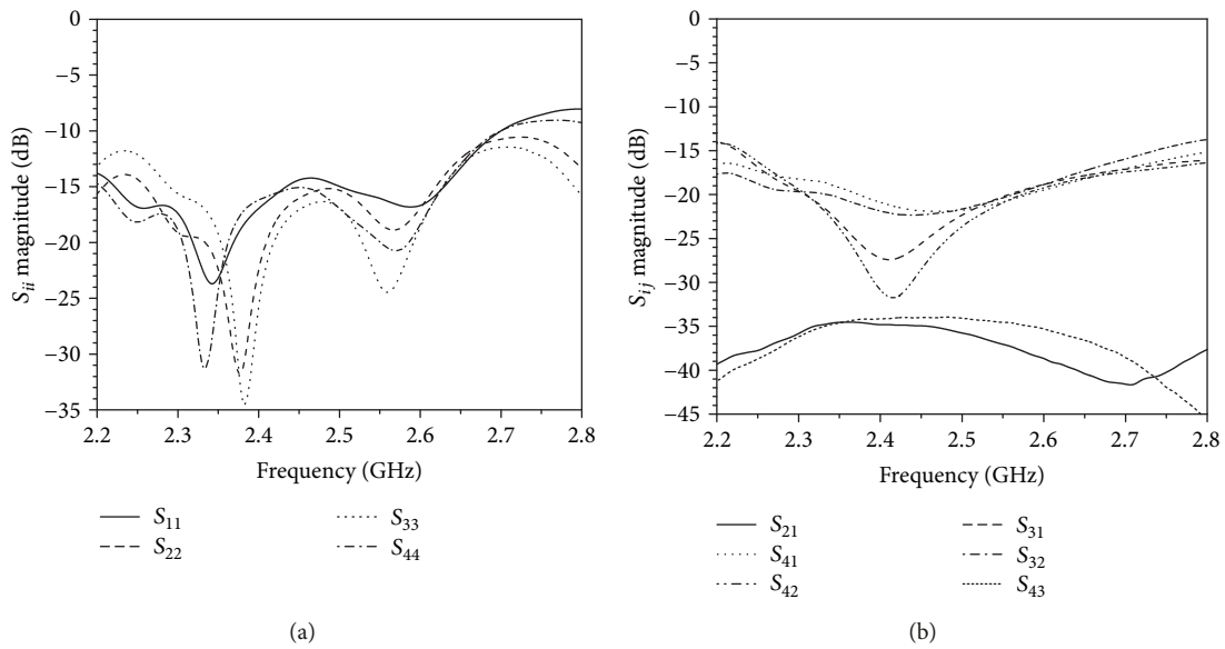
FIGURE 6: Measured magnitude of (a) the return losses and (b) the isolation coefficients of the 4 \times 4 BM.
