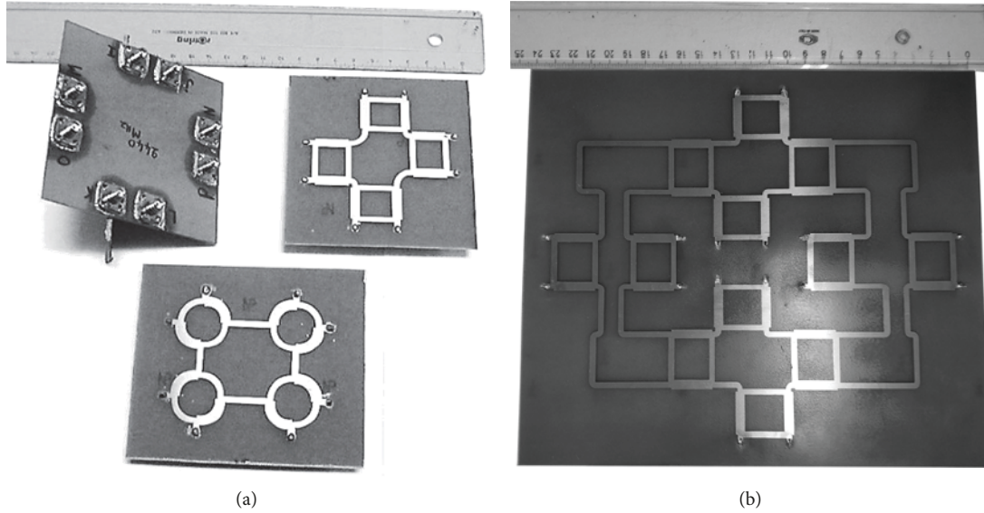
FIGURE 5: Pictures of certain fabricated prototypes. (a) Top view of the 4 \times 4 BMs that correspond to the layouts of Figures 2(b) and 2(c) and bottom view of the layout depicted in Figure 2(b). (b) Top view of the 8 \times 8 BM.
