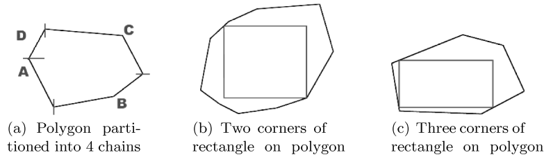
Fig. 8. Process for finding the largest inscribed rectangle in a polygon.
