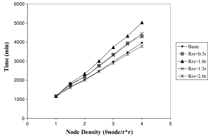
Fig. 28. Half-life for reference point scattering.
