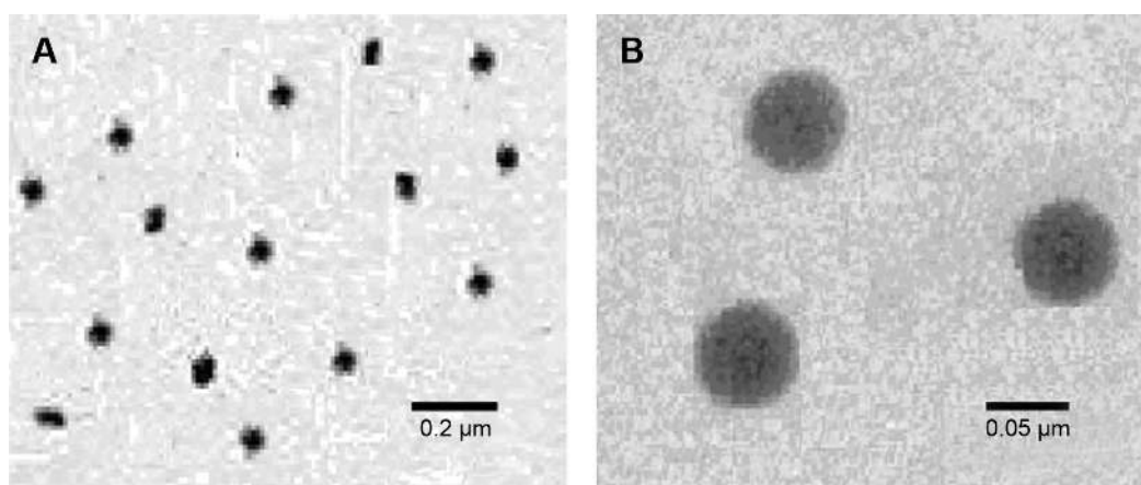
Figure 3 TEM images of the nanoemulsion in the different scale of 0.2 \mu\text{m} (A) and 0.05 \mu\text{m} (B). Abbreviations: SNEDDS, self-nanoemulsifying drug delivery system; TEM, transmission electron microscopy.
