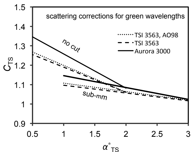
Fig. 5. Total scattering correction functions for the green wavelengths. Shown are two branches for no cut and sub- \mu m cut.
