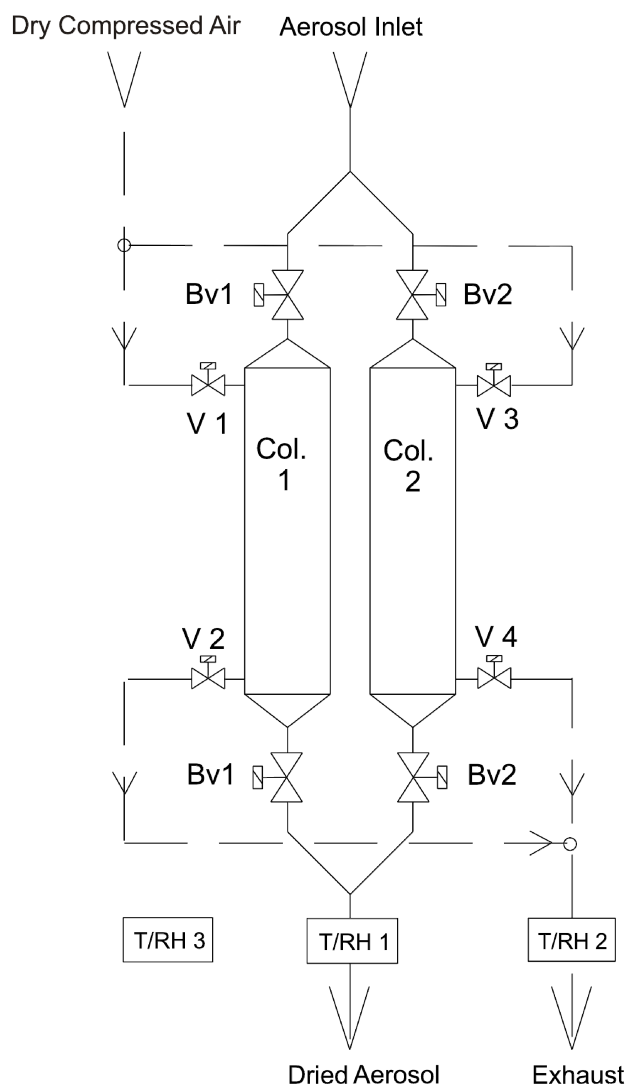
Fig. 1. Schematic view of the aerosol dryer.
