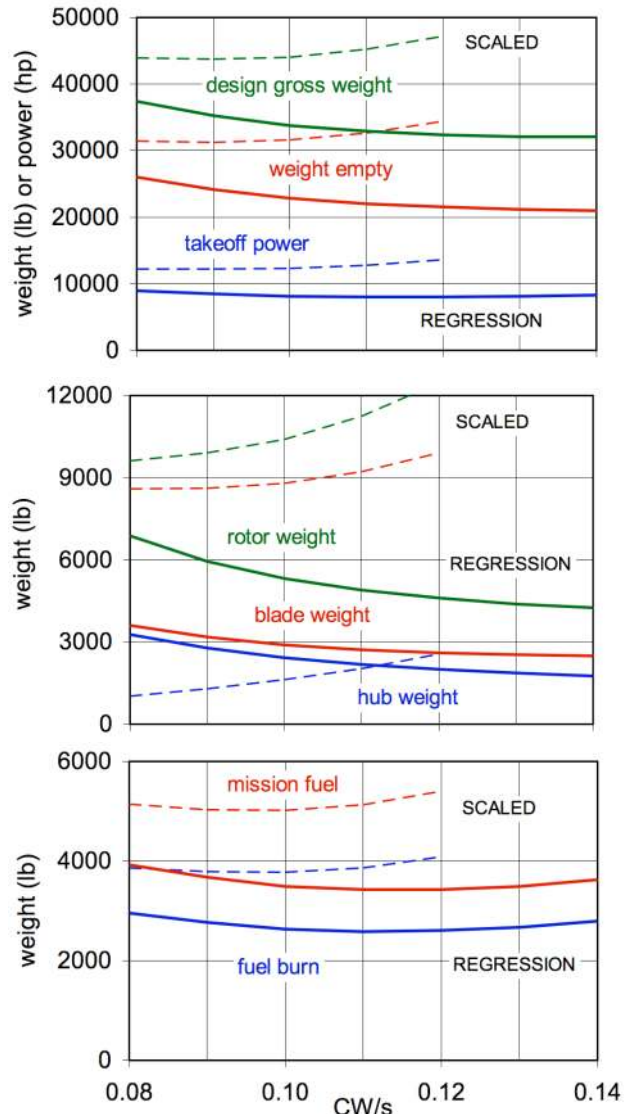
Figure 21. Variation of civil aircraft design with blade loading C_W/\sigma (disk loading 16 \text{ lb/ft}^2 for scaled rotor weight model, 12 \text{ lb/ft}^2 for regression rotor weight model).
