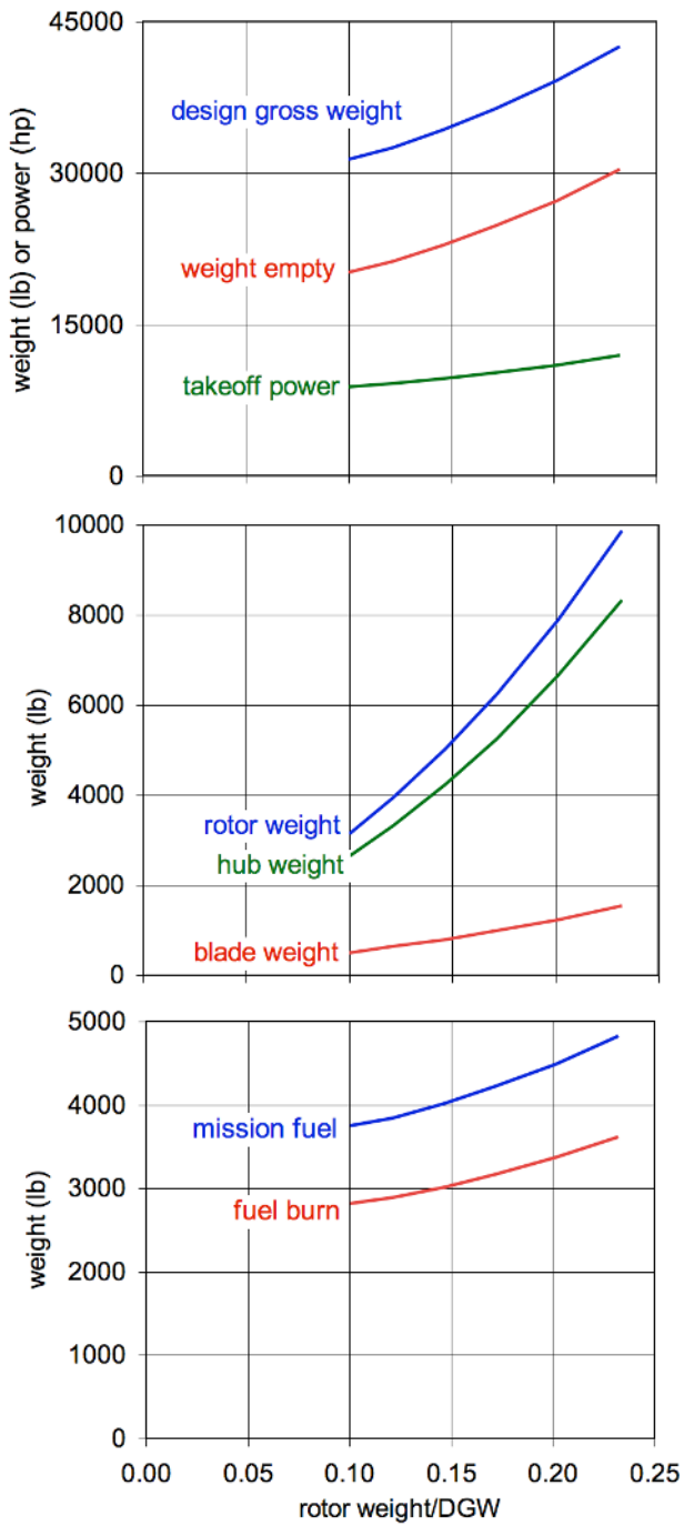
Figure 38. Influence of rotor weight technology (rotor weight fraction of design gross weight) on civil aircraft with scaled rotor weight model.
