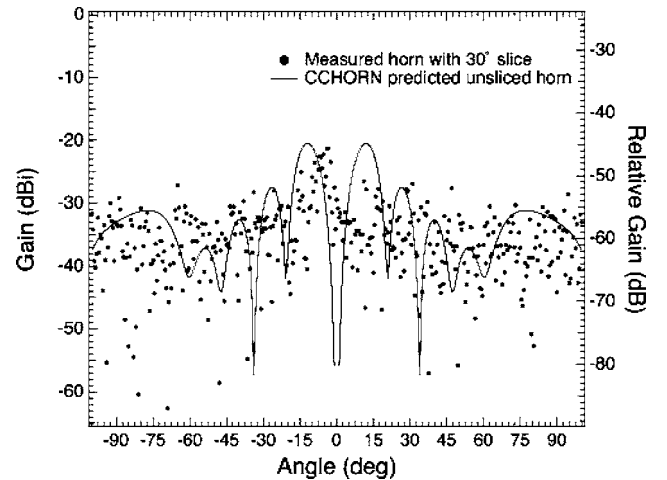
FIG. 6. Predicted and measured cross-polar response for the 10 GHz horn at 10.11 GHz. The measured response is near or below the noise floor of the measurement at most angles.
