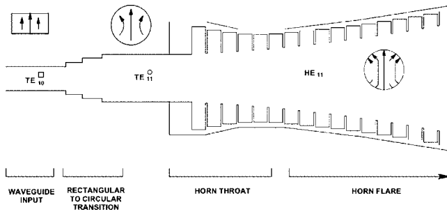
FIG. 1. Schematic of the horn system.
