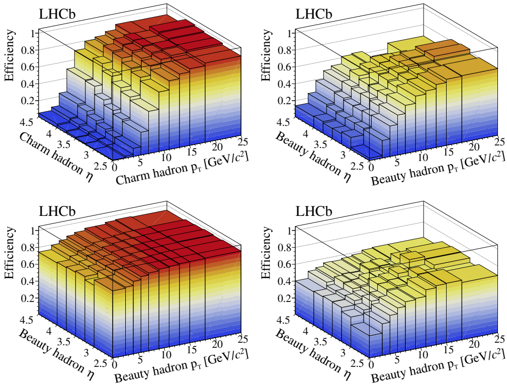
Figure 23. Two-dimensional efficiencies of the L0 trigger lines in Run 2 data: (top left) L0 hadron; (top right) L0 electron; (bottom left) L0 muon; and (bottom right) L0 dimuon. The L0 hadron efficiency is evaluated using D^0 \rightarrow K^- \pi^+ decays, whereas the others are evaluated using the relevant signals listed in figure 20 and figure 21.
