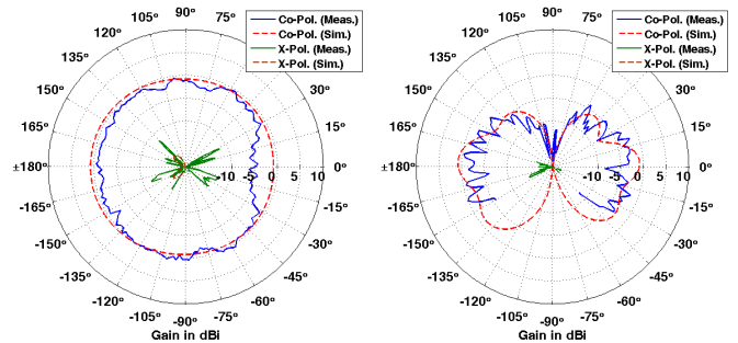
Fig. 7. Gain of the folded slot antenna: (a) H-Plane. (b) E-Plane.
