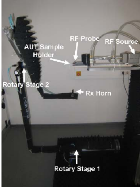
Fig.4. Antenna measurement setup
