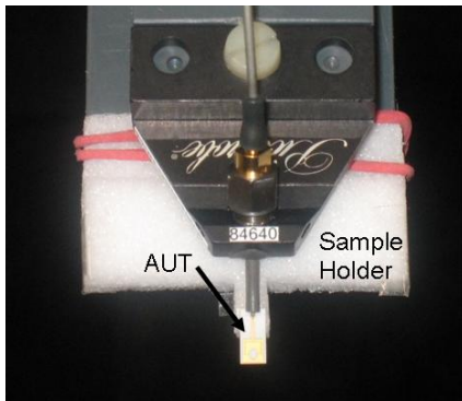
Fig. 5. AUT sample holder and RF probe
