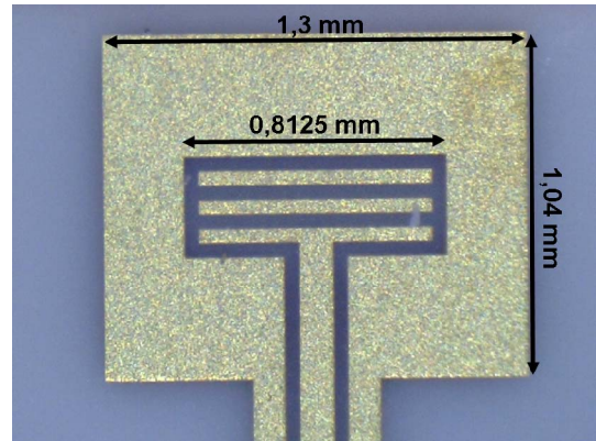
Fig. 2. Folded slot antenna
