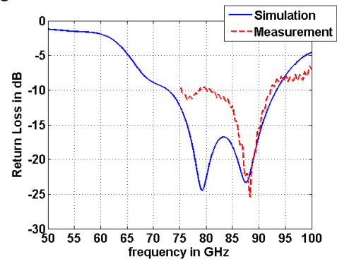
Fig. 6. Return Loss of the folded slot antenna
