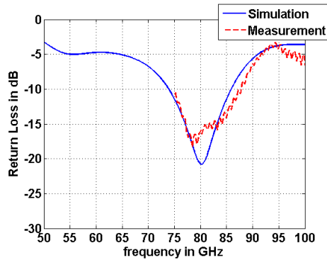
Fig. 8. Return Loss of the dual bow-tie antenna
