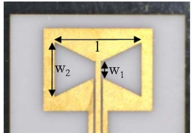
Fig. 3. Dual bow-tie antenna
