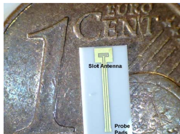
Fig. 1. Slot antenna, feeding lines and probe pads
