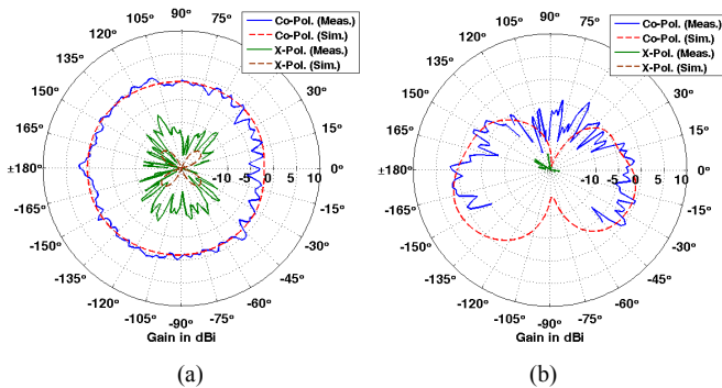
Fig. 9. Gain of the dual bow-tie antenna: (a) H-Plane. (b) E-Plane.
