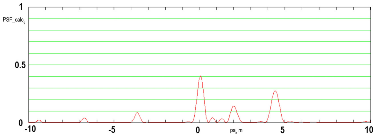
Figure 3. Theoretical PSF cross-section for the new multifocal IOL with a 3.0 mm pupil diameter ( pa_q \cdot \text{mm} = defocus addition in arbitrary units; \text{PSF\_calc}_q = calculated point-spread function).
