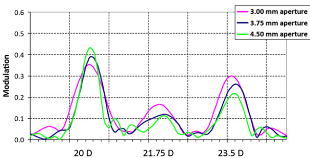
Figure 7. The MTF peaks at 50 cycles/mm for an aperture of 3.75 mm.
