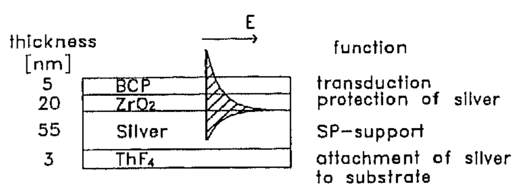
Fig. 3. SP supporting structure, showing thickness and function of the layers.
