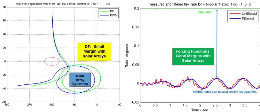
Figure 17. Stability Analysis shows Solar Array Flex Non-Compliance with DF-derived Sufficient Condition, but Adequate Margins Using less-Conservative Forcing Function Approach
