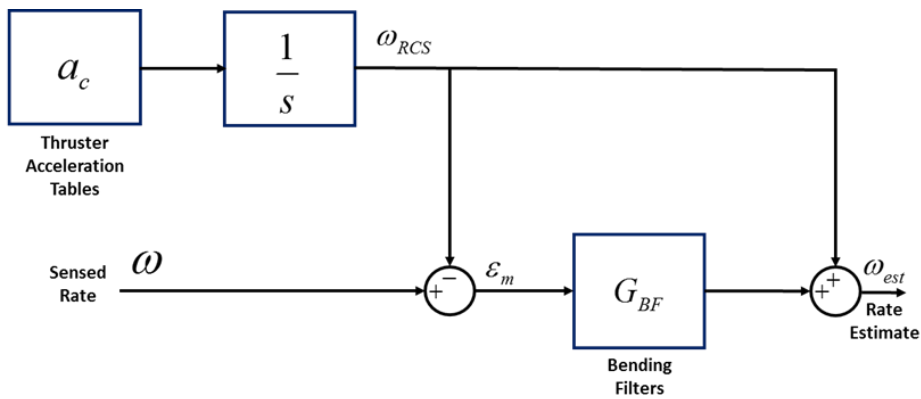
Figure 21. Shuttle Conceptual Implementation of Rate Estimation Using Feed-Forward
