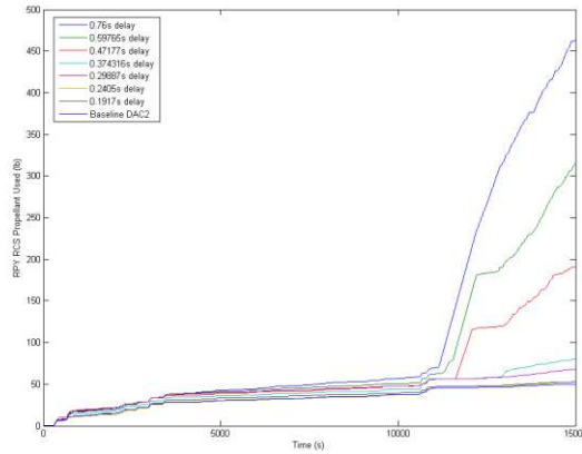
Figure 20. Propellant Usage for Differing Filter Lag Times
