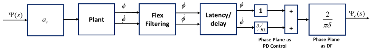
Figure 11. Simplified Phase Plane Control System with Phase Plane Modeled as PD/Relay Combination
