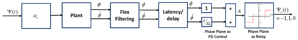
Figure 10. Simplified Phase Plane Control System with Phase Plane Modeled as PD/Relay Combination
