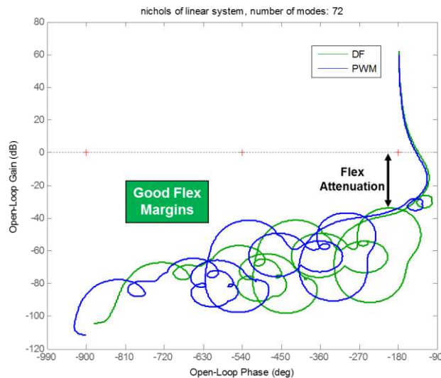
Figure 16. Flex Body Stability Results: Adequate Flex Margins Demonstrated by both DF and PWM Approaches
