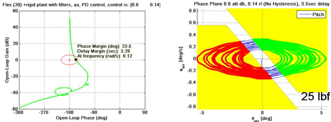
Figure 13: Time domain Simulation Showing Good Agreement with Rigid Body Margin Predicted by Describing Function Representation of Phase plane. Unstable control (right) with 3.5 second latency.
