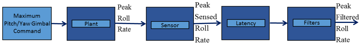
Figure 23. System Producing Peak Steady State Roll Flex Rate Given Worst Case Pitch/Yaw TVC Input
