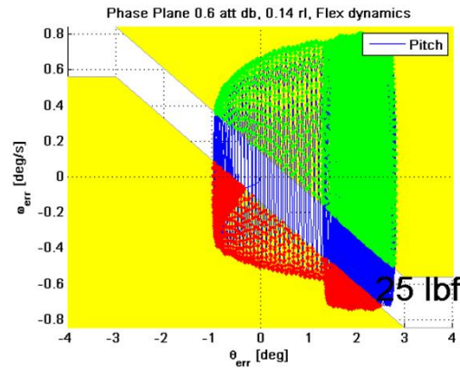
Figure 15. Phase Plane Flex Induced Instability, Colors Denote Firing Command Directions: Green = -1, Blue = 0 (Off), Red = +1
