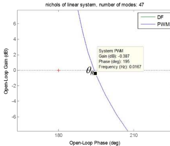
Figure 14. Graphically Determining Allowable Latency ( T_D ) Given Rigid Body Phase Margin ( \theta_R ) and Rigid Body Cross-Over Frequency
