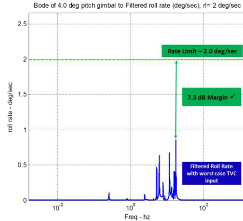
Figure 24. Example Showing Peak Steady State Flex Body Roll Rate within Phase Plane Rate Limit for a Peak Pitch/Yaw Gimbal Excitation
