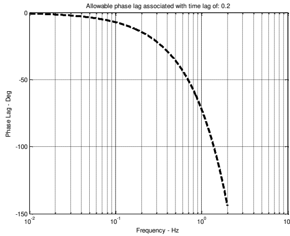
Figure 19. Filter Phase Design Constraint for allowable filter lag of 0.2 seconds.
