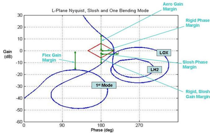
Figure 6. Typical Stability Margin Definitions
