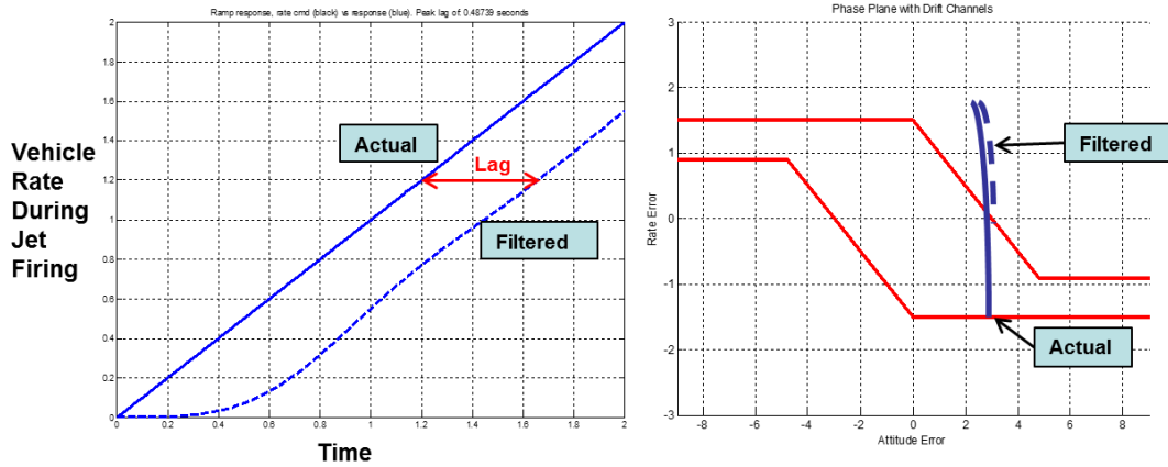
Figure 18. Filter Induced Lag Results in Phase Plane Overshoot
