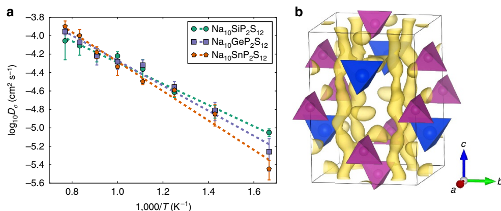
Figure 2 | DFT computed diffusivity of Na 10 SnP 2 S 12 . (a) Na-diffusivity in Na 10 SiP 2 S 12 , Na 10 GeP 2 S 12 and Na 10 SnP 2 S 12 from AIMD simulation. Dashed lines are Arrhenius fits to the data, and error bars are standard error of the mean. (b) Na-ion probability density isosurface (yellow) of Na 10 SnP 2 S 12 from 600 K AIMD simulation. SnS 4 tetrahedra are marked in blue, PS 4 tetrahedra in purple.
