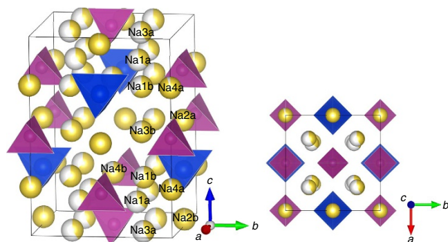
Figure 1 | Structure of Na 10 SnP 2 S 12 from DFT calculations. Sodium occupancies are calculated from 600 K AIMD simulation (see Methods). All ground-state NMPS structures share this M/P ordering, which reduces the symmetry from the P4_2/nmc space group to P\bar{4}m2 , separating each Na-site into two symmetrically distinct but similar sites marked as a and b . PS 4 tetrahedra are marked in purple, SnS 4 tetrahedra in blue and Na-sites in yellow. The ground-state Na-ordering is shown in Supplementary Fig. 2.
