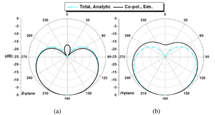
Fig. 11 Normalized radiation patterns in the E- and H-planes for the backwards radiating Huygens source antenna at its resonance frequency f_0 = 1.505 GHz.
