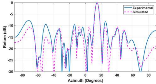
Fig. 12 Target at 15 degrees; range-angle map
