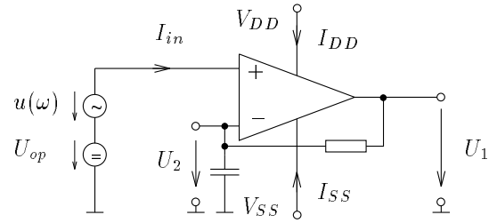
Figure 2: Test configuration for testing the operational amplifier.
