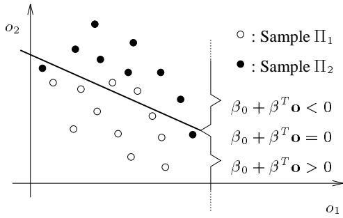
Figure 4: Allocation rule.
