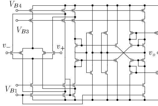
Figure 1: CMOS operational amplifier to be tested.
