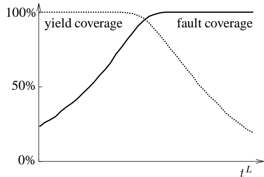
Figure 5: Trade off between yield coverage and fault coverage for specification SR_- (2000 training samples).
