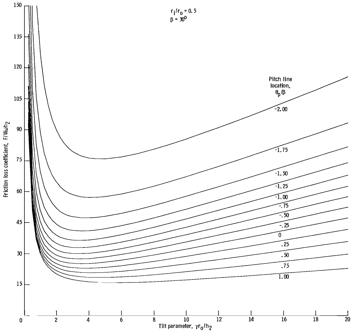
(c) Friction loss.
