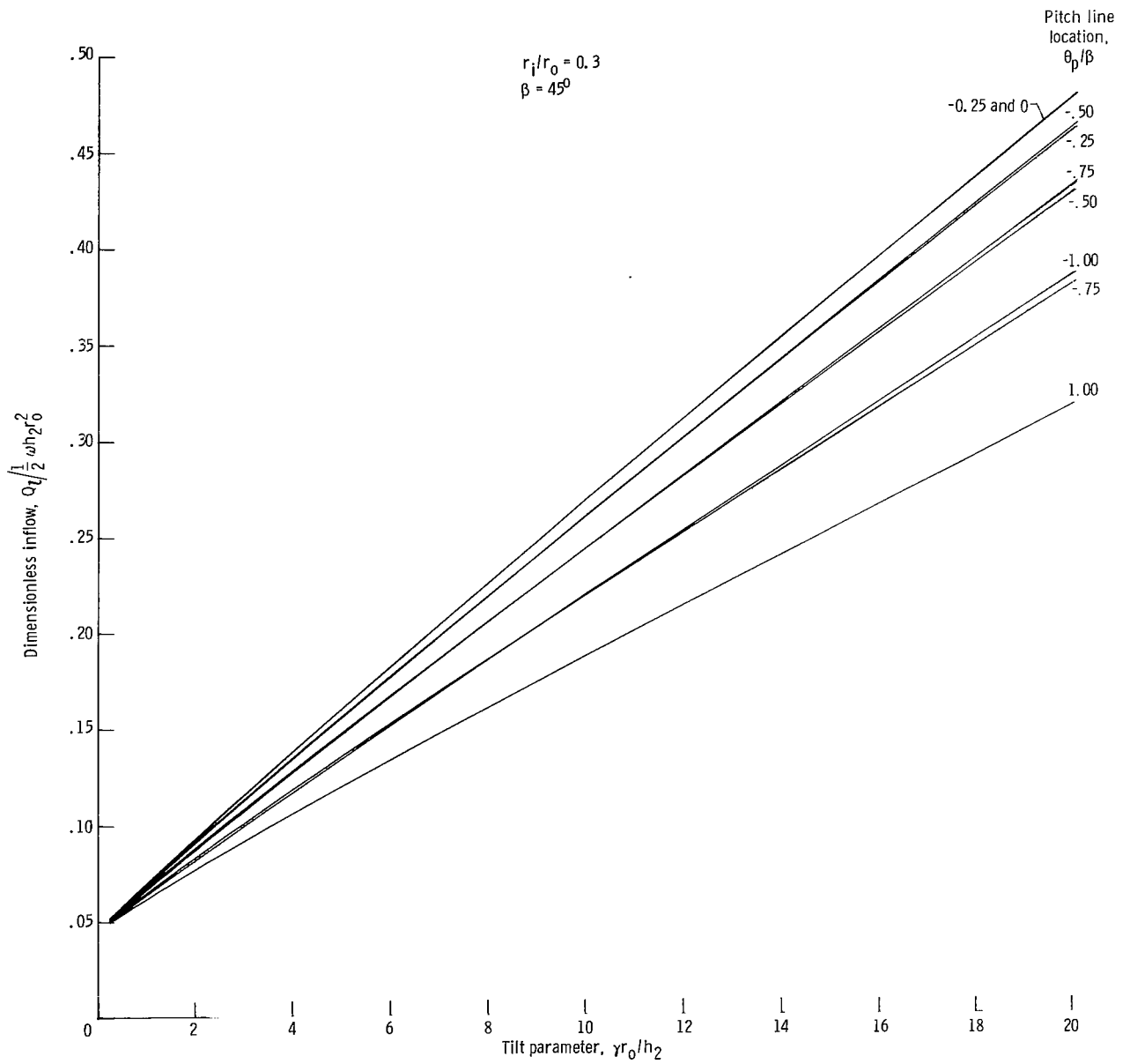
(d) Lubricant inflow. Figure 4. - Continued.
