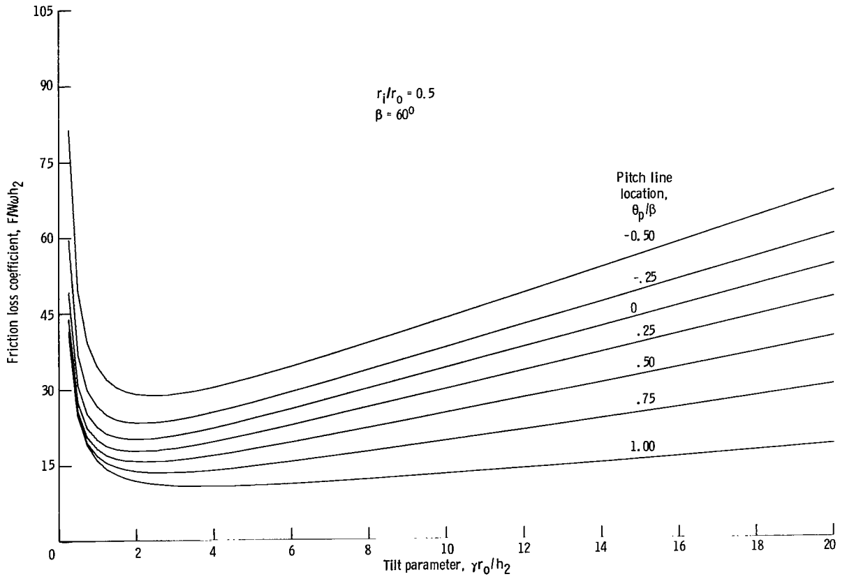
(c) Friction loss.
