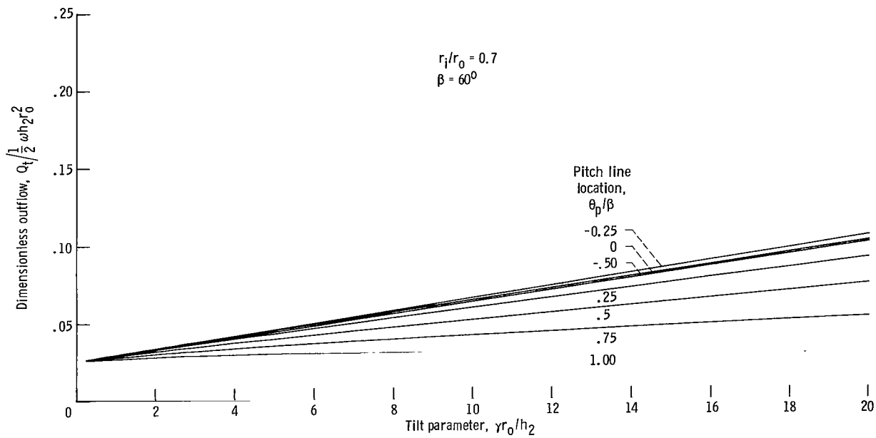
(e) Lubricant outflow at trailing edge.
