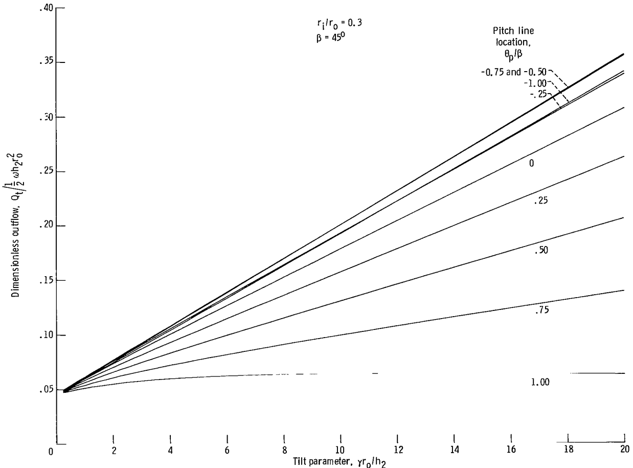
(e) Lubricant outflow at trailing edge.
