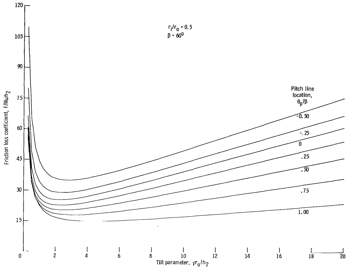
(c) Friction loss.
