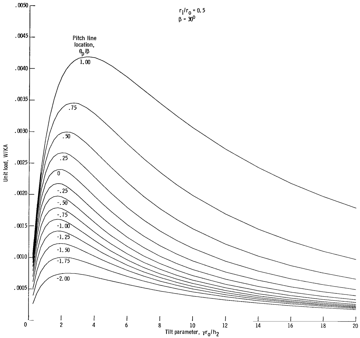
(b) Load capacity.
