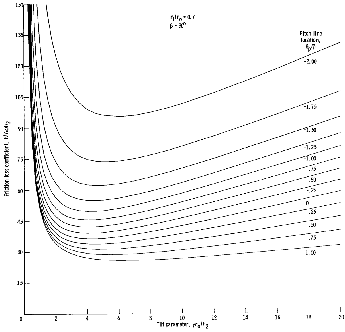
(c) Friction loss. Figure 9. - Continued.
