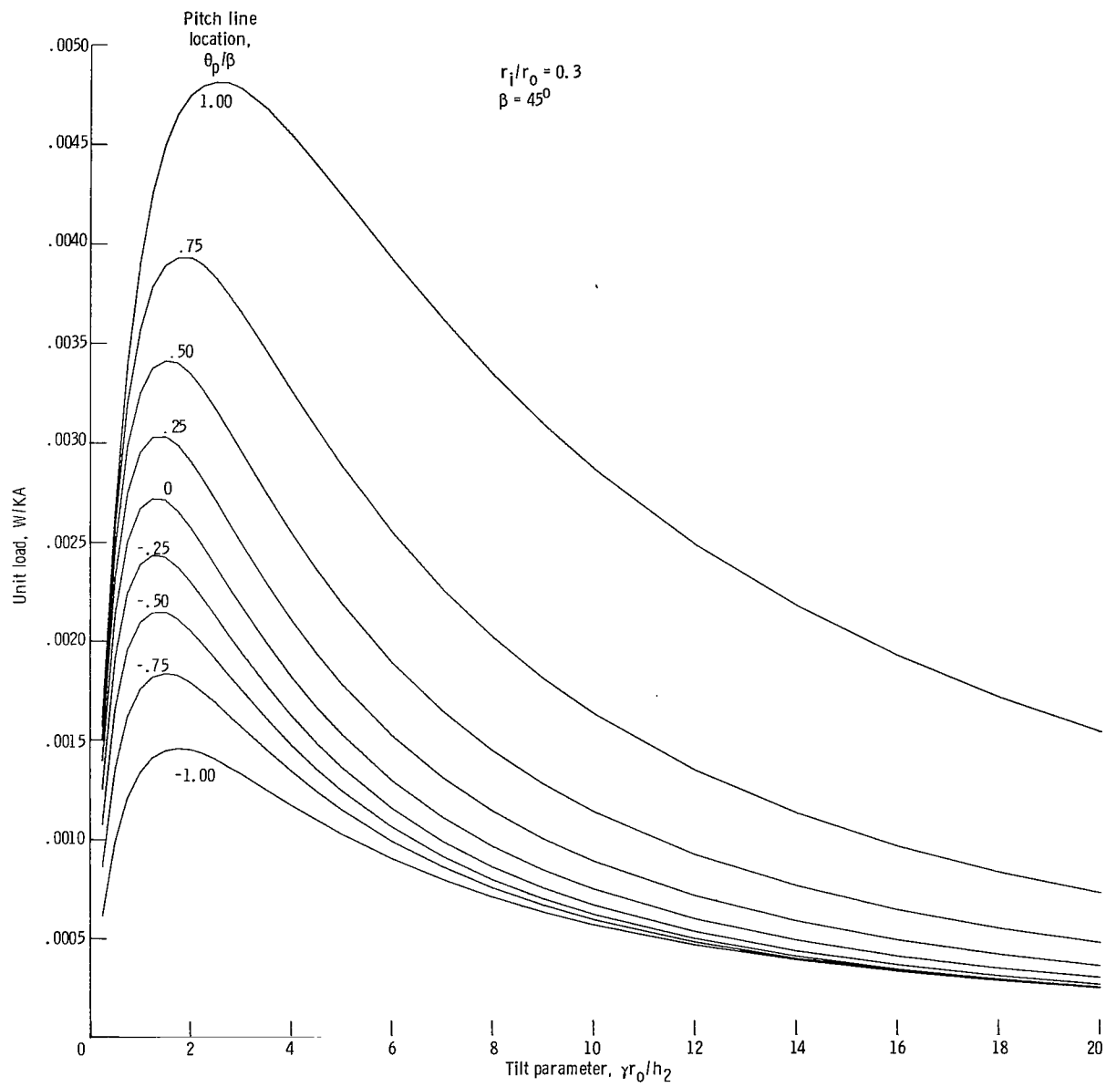
(b) Load capacity.
