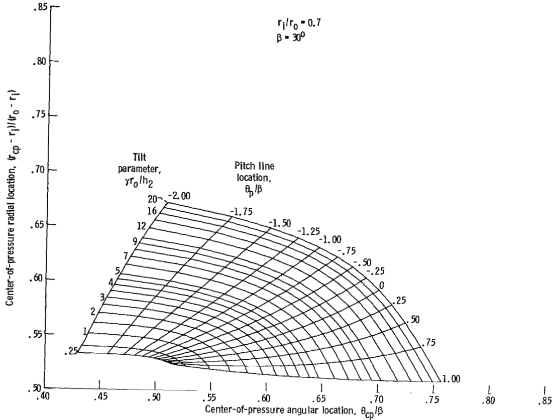
Figure 9. - Design charts for flat, sector-shaped pad with ratio of inner to outer radius r_i/r_o of 0.7 and angular extent \beta of 30^\circ .
