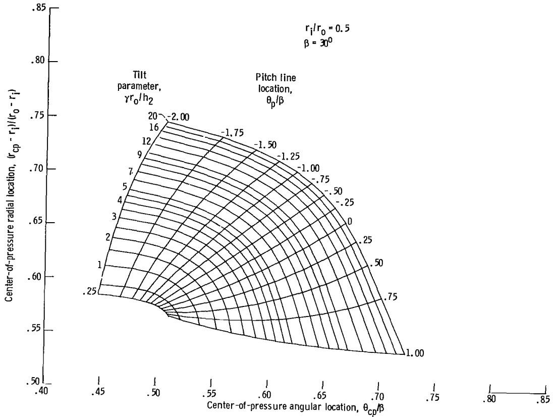
Figure 6. - Design charts for flat, sector-shaped pad with ratio of inner to outer radius r_i/r_o of 0.5 and angular extent \beta of 30^\circ .
