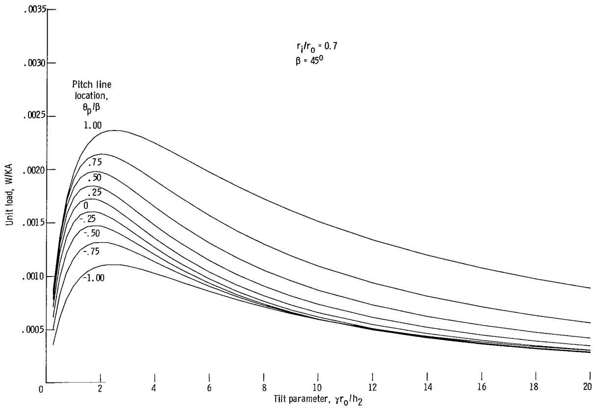
(b) Load capacity.
