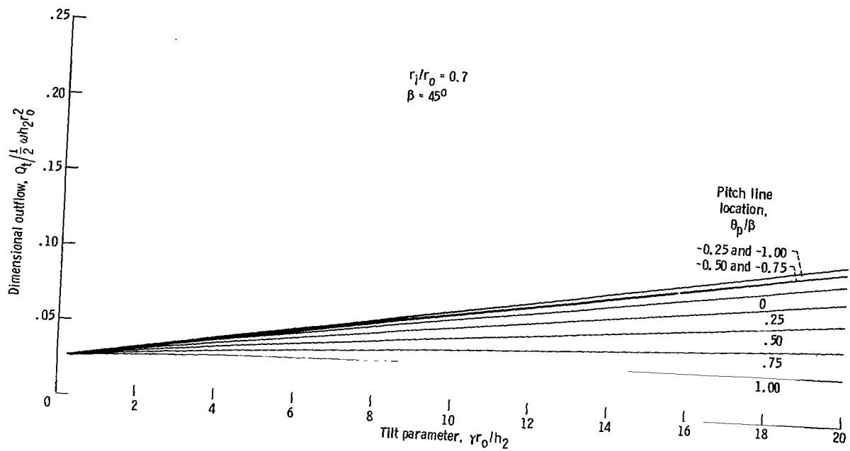
(e) Lubricant outflow at trailing edge.
