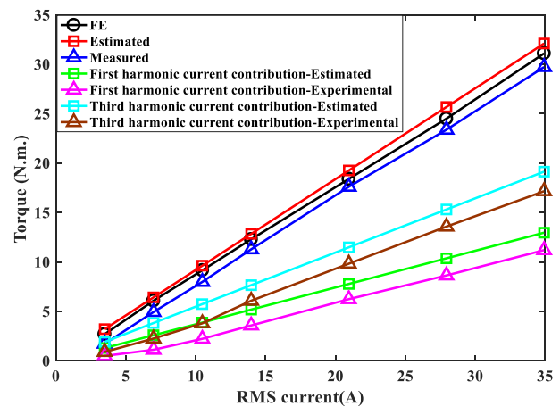
Fig. 10. Comparison of the mean value of torque between measured values, estimated values and FE calculation.
