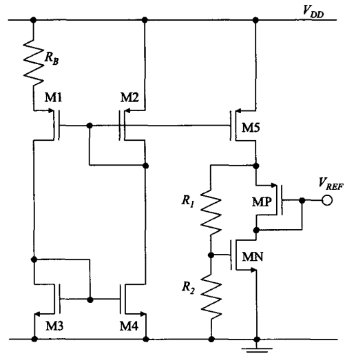
Fig. 15: A voltage reference in standard CMOS technologies proposed by Leung et al. [21], [22].
