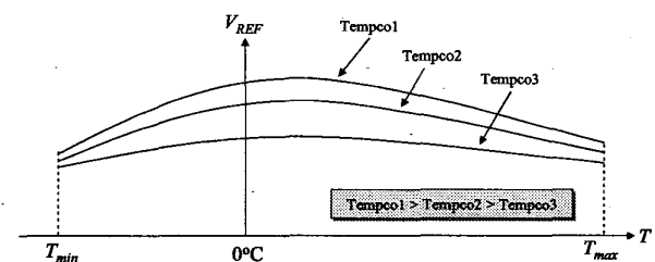
Fig. 5: Reference voltage using different resistor materials.
