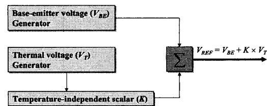
Fig. 2: Concept of bandgap voltage reference.
