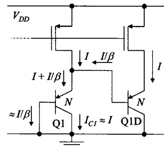
Fig. 7: A circuit for base-current compensation.
