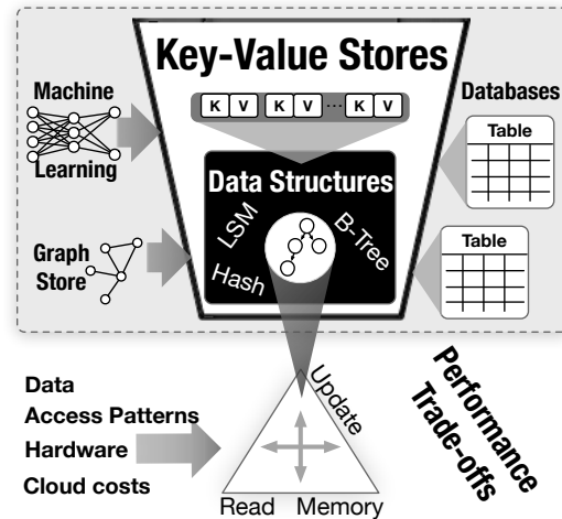
Figure 1: From performance trade-offs to data structures, key-value stores and rich applications.
