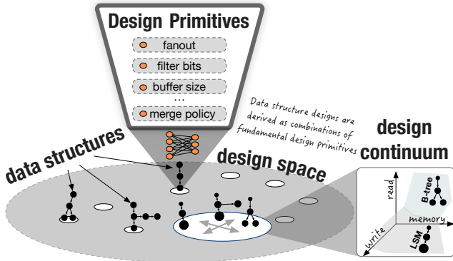
Figure 2: From data layout design principles to the design space of possible data structures, where design continuums can be observed to help navigate performance trade-offs across diverse data structure designs.
