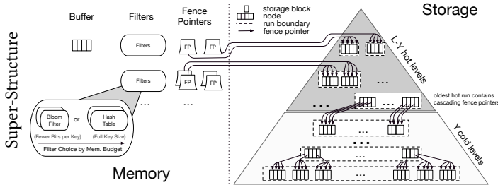
Figure 6: Extending the design continuum to support Log Structured Hash table designs.
