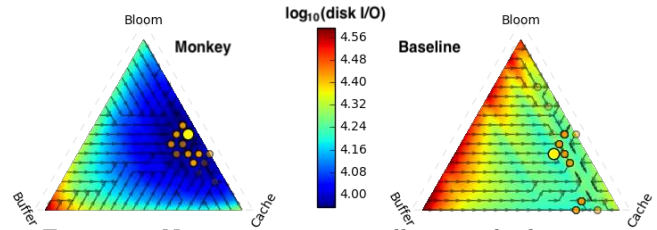
Figure 11: Navigating memory allocation by learning.
