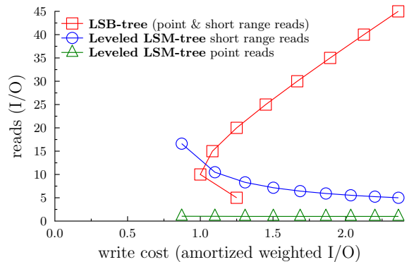
Figure 8: Leveled LSM-tree dominates LSB-tree for most of their respective continuums.
