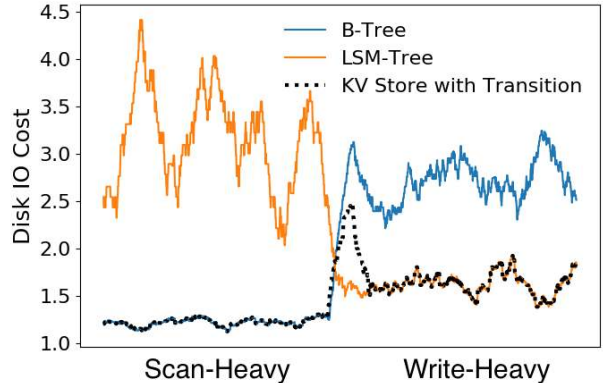
Figure 10: Potential benefit of on-the-fly transitions between B + tree and LSM-tree.
