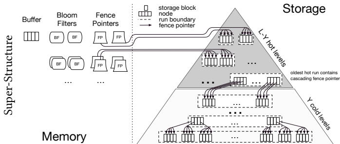
Figure 3: An example of a design continuum: connecting complex designs with few continuous parameters.
