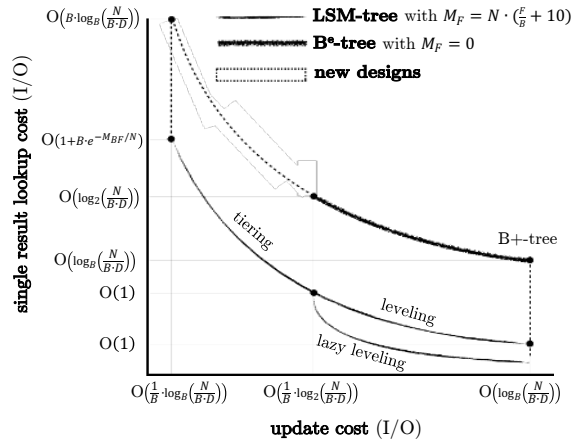
Figure 9: Visualizing the performance continuum.
