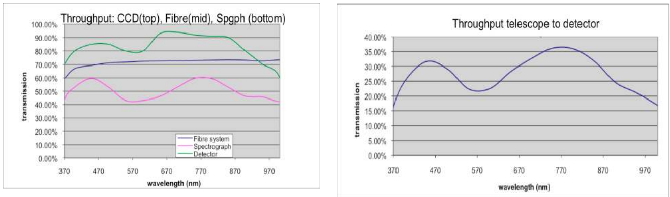
Figure 4. Throughput estimates for the R=5,000 mode of the WHT MOS. Left : top to bottom, the contributions of detector, fibre and spectrograph. Right : total throughput from the telescope to the detector.
