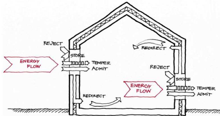
Figure 1. Illustration of the dynamic energy flows and interactions in buildings with adaptive/responsive facades (from: IEA EBC Annex 44, adapted by Fernández Solla [9]). The energy flows from outside to inside and vice versa can actively be influenced by the adaptive façade technologies (reject, store, temper, admit, redirect, etc.).
