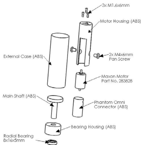
Figure 1. Exploded view of stylus and drive system
