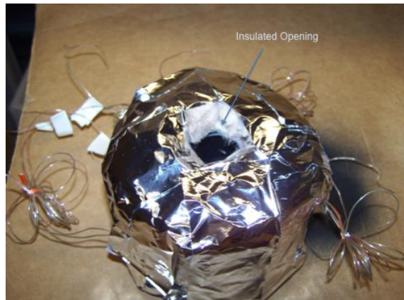
Figure 5. Fully insulated calorimeter with light opening.
