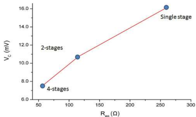
Fig. 4. V_C as function of the equivalent resistance R_{EQ} for constant P_r = -30 dBm. Increasing R_{EQ} by decreasing the numbers of stages N will increase V_C .
