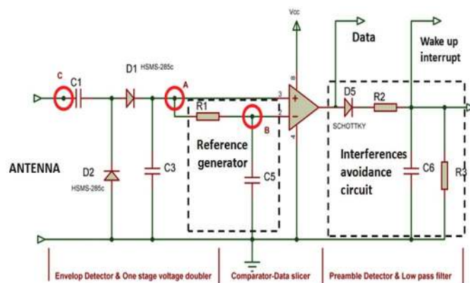
Fig. 5. Nanopower high-sensitivity WUR architecture.
