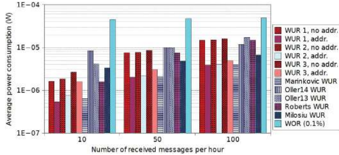
Fig. 12. Average power consumption of the communication with proposed WURs and recently published WURs, compared to the duty-cycled radio (WOR) with 0.1% duty cycle, taking into account that Roberts WUR and Oller13 WUR do not have addressing possibilities.
