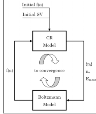
Figure 1. Schematics of the Quick Source cycle.
