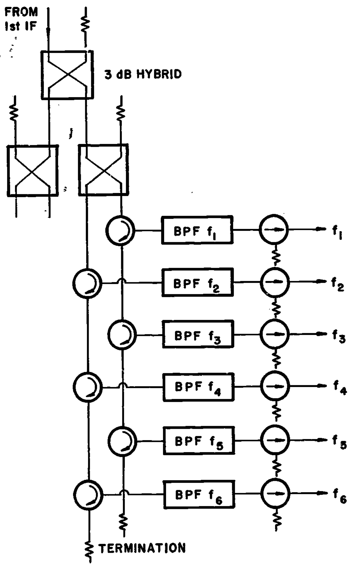
Fig. 13 Branching Network
