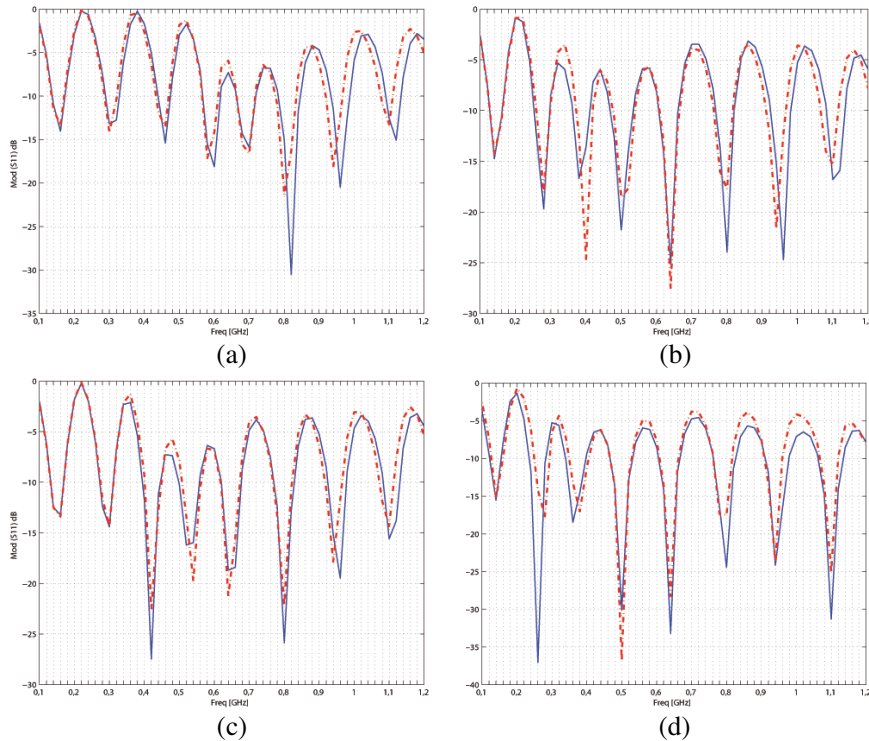
Figure 7. Frequency response of the Modulus of S_{11} at the feeded port of balun (fed in unbalanced way by a coaxial cable). Blu line: Monolithic antenna; Red line: Discretised reconfigurable antenna. (a) Antenna in free-space. (b) Antenna on half space with relative dielectric permittivity 4. (c) Antenna on half-space with relative dielectric permittivity 9. (d) Antenna on half-space with relative dielectric permittivity 16.
