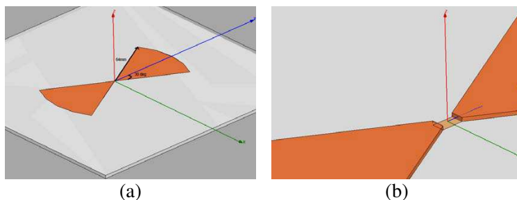
Figure 2. (a) Reference bow-tie antenna: thickness 36 mm, radius 64 mm and flared angle 30 degree, placed on substrate epoxy FR4 with extent 20 cm × 20 cm × 3 mm. (b) Zoom of the feeding zone.
