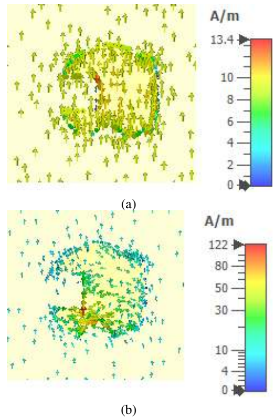
FIGURE 8. Surface current distribution of unit cell at: (a) 5.5 GHz (b) 20 GHz.
