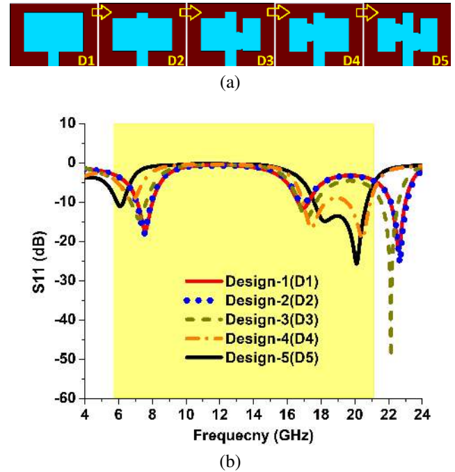
FIGURE 2. Antenna element: (a) design evolution stages (b) S-parameter comparison.
