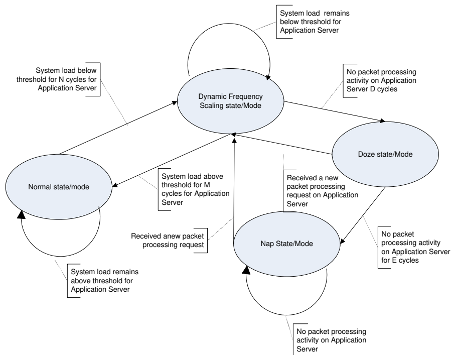
Figure 12: DPC State machine for the dedicated data plane cores
