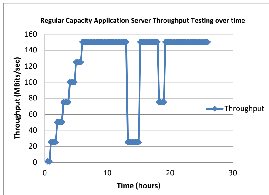
Figure 14: Throughput Testing Rate over a Period of Time
