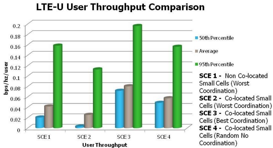
Figure 6: LTE-U User Throughput Comparison
