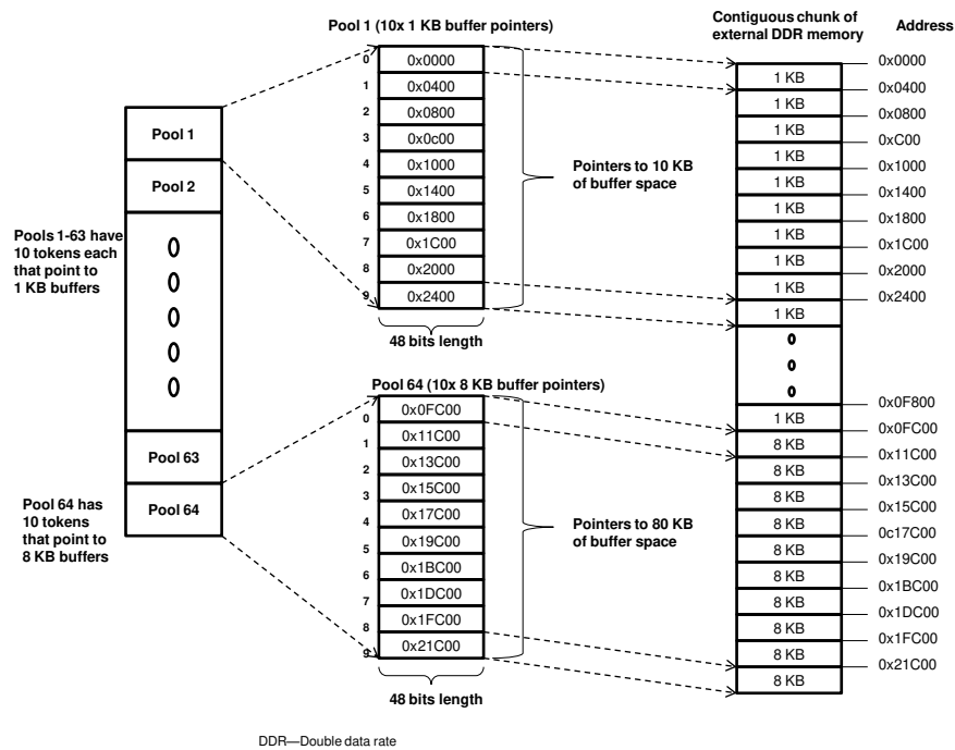
Figure 16: P4080 BMAN Buffer Pool Seeding
