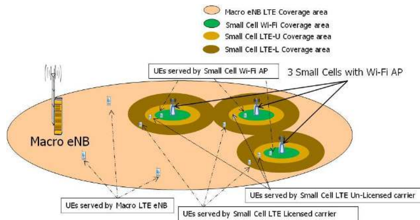
Figure 1: Single Operator LTE-U Deployment Scenario in a Wireless HetNet
