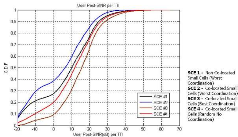
Figure 5: LTE-U SINR Distribution Comparison
