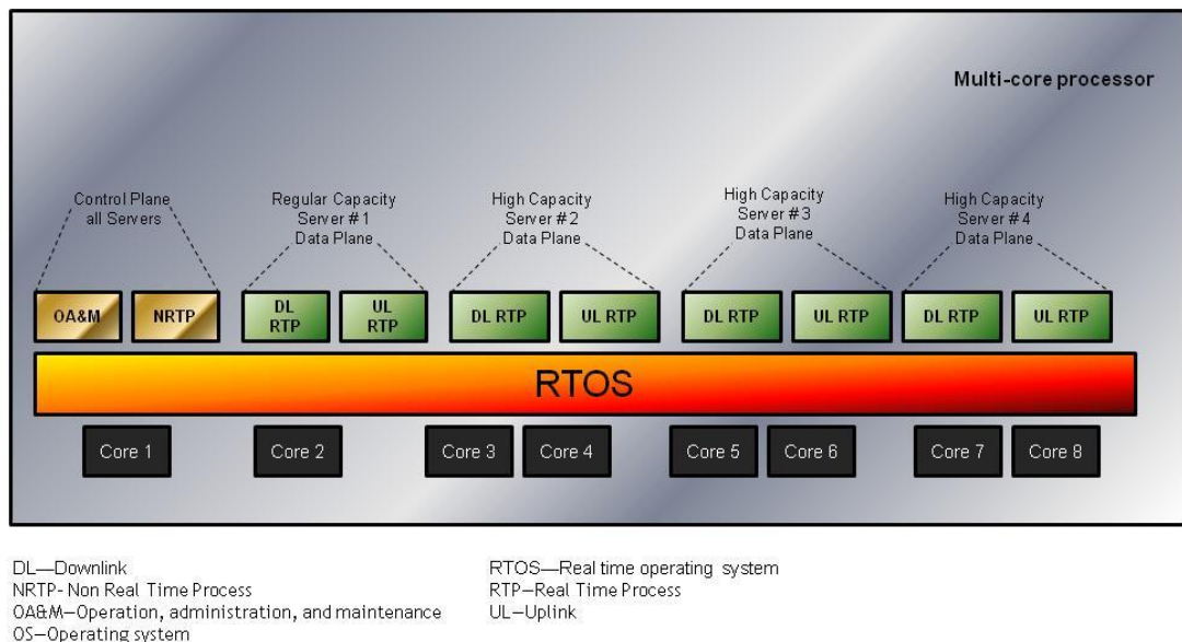
Figure 9: Symmetric Multi-Processing (SMP) Configuration
