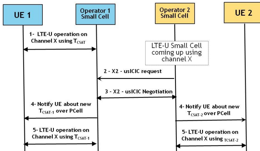
Figure 4: Event Trace Diagram for the proposed usICIC Mechanism
