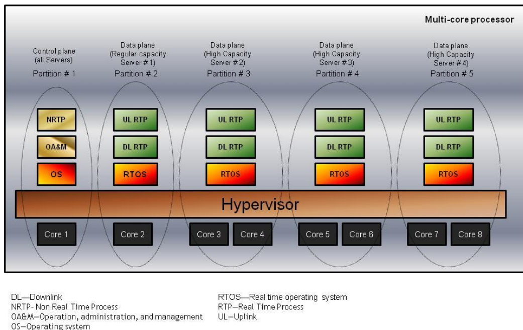
Figure 8: Supervised Asymmetric Multi-Processing (S-AMP) Configuration
