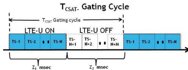
Figure 2: TCSAT Gating Cycle for LTE-U Channel Sharing with Wi-Fi
