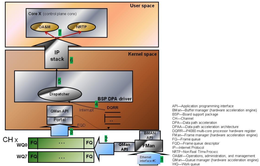
Figure 17: Ingress Control Plane IP Packet processing using Protocol Stack
