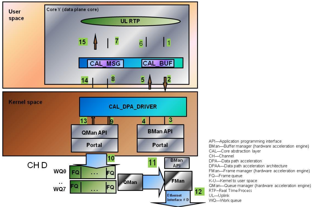
Figure 20: Egress Data Plane IP Packet Processing
