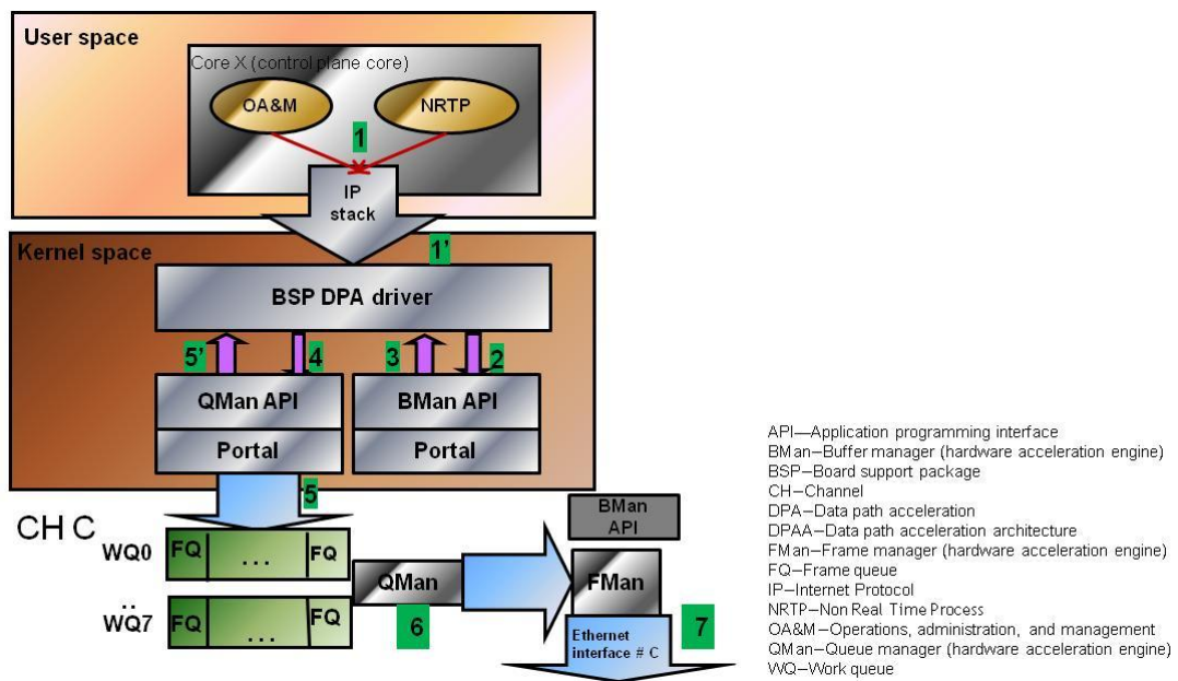
Figure 18: Egress Control Plane IP packet Processing using the Protocol Stack
