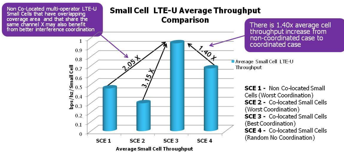
Figure 7: LTE-U Small Cell Average Throughput Comparison
