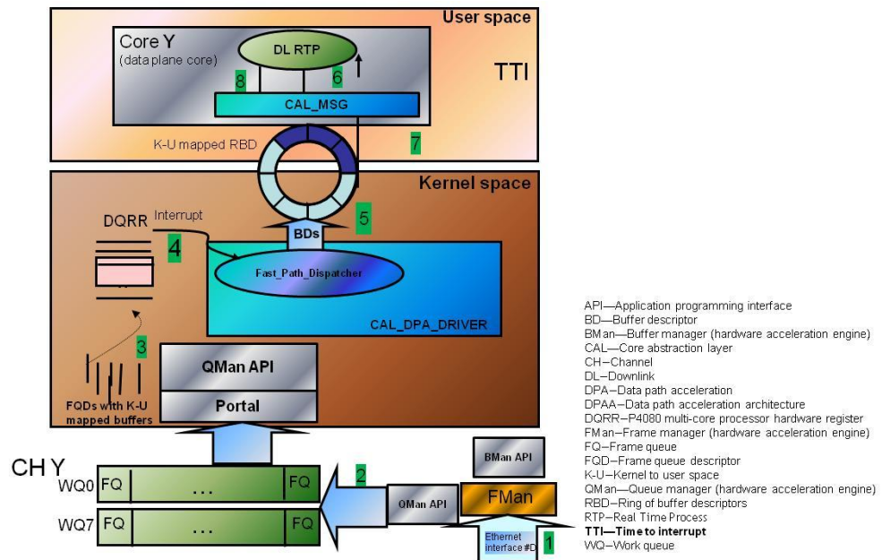
Figure 19: Ingress Data Plane IP Packet Processing
