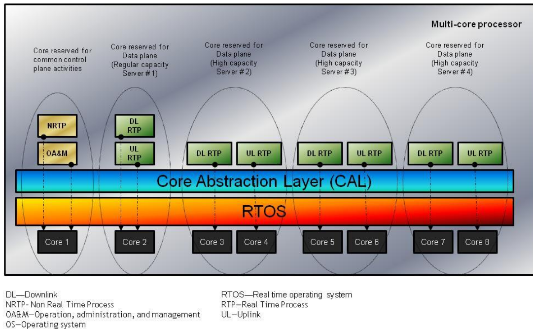
Figure 10: Deterministic Symmetric Multi-Processing (D-SMP) Configuration
