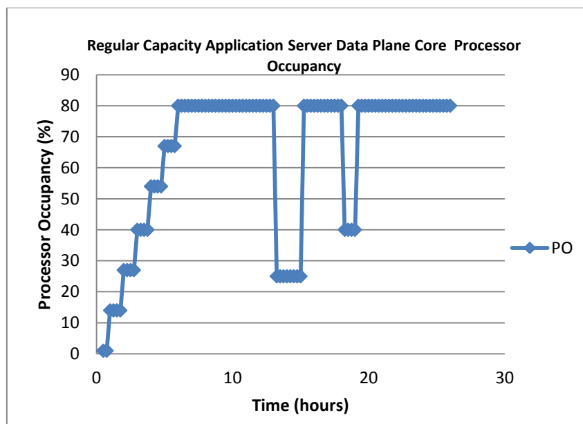
Figure 15: Processor Occupancy Load Corresponding To Throughput Rate
