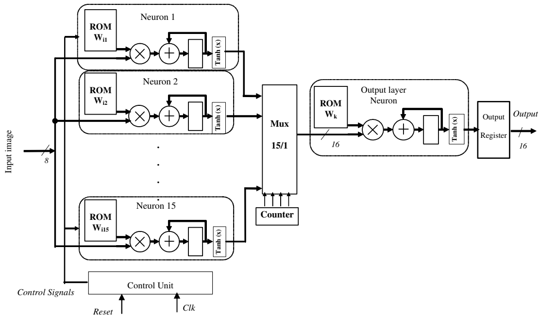
Fig.3: Block diagram
