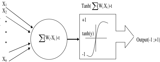
Fig.1: The neuron of supervised training [8]
